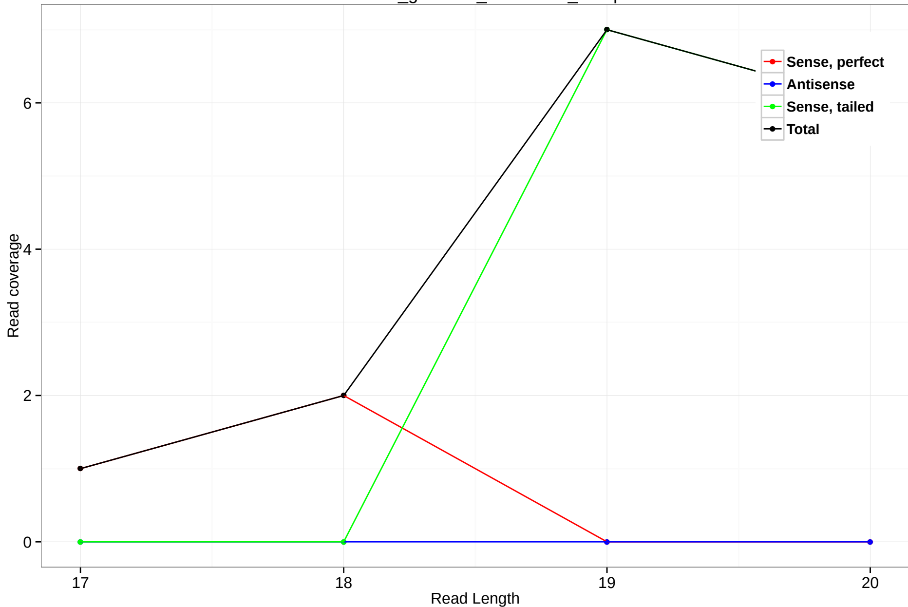
rheMac3_genscan_chr1.4582_10.5p
