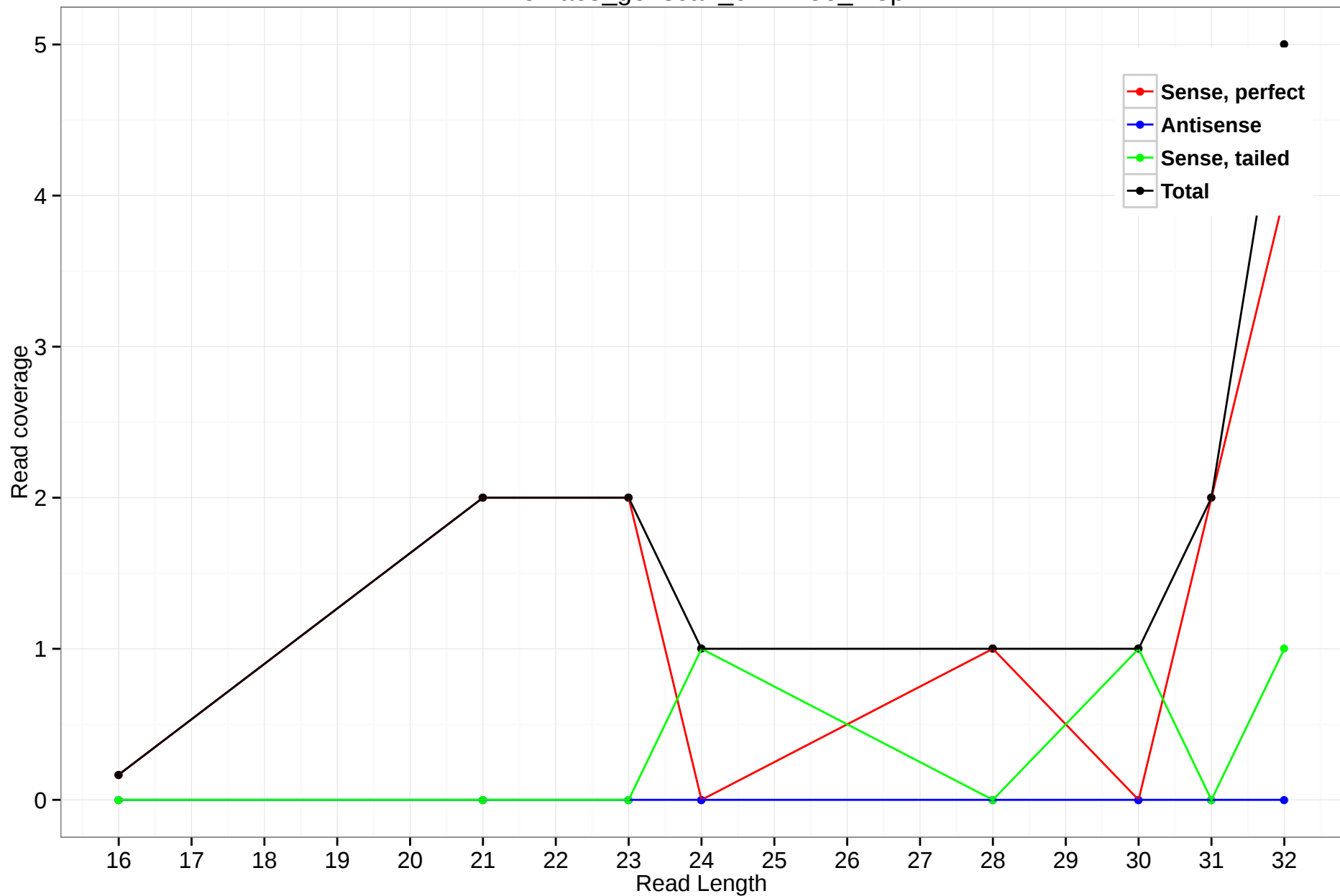
rheMac3_genscan_chr1.456_4.5p
