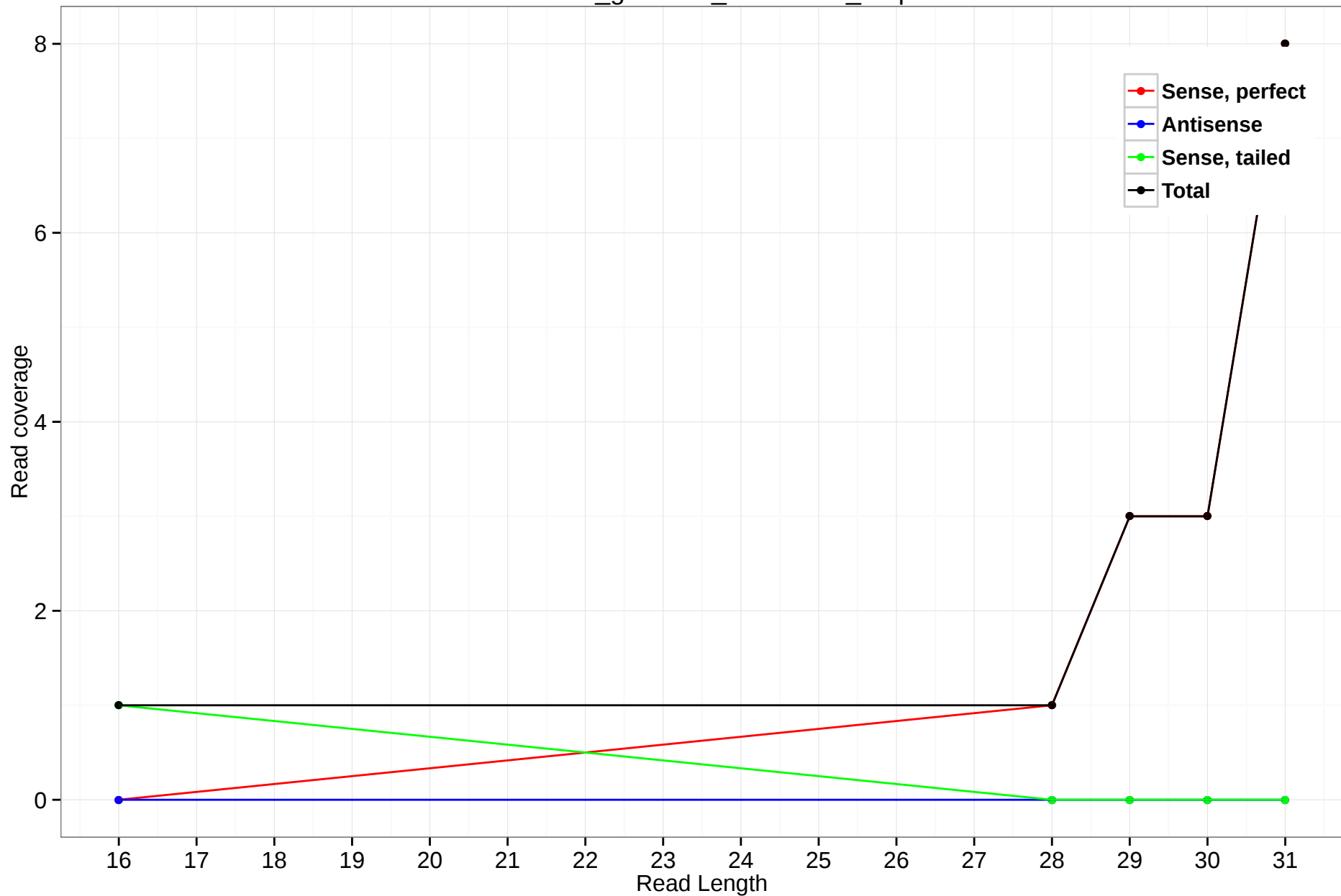
rheMac3_genscan_chr1.4535_1.3p
