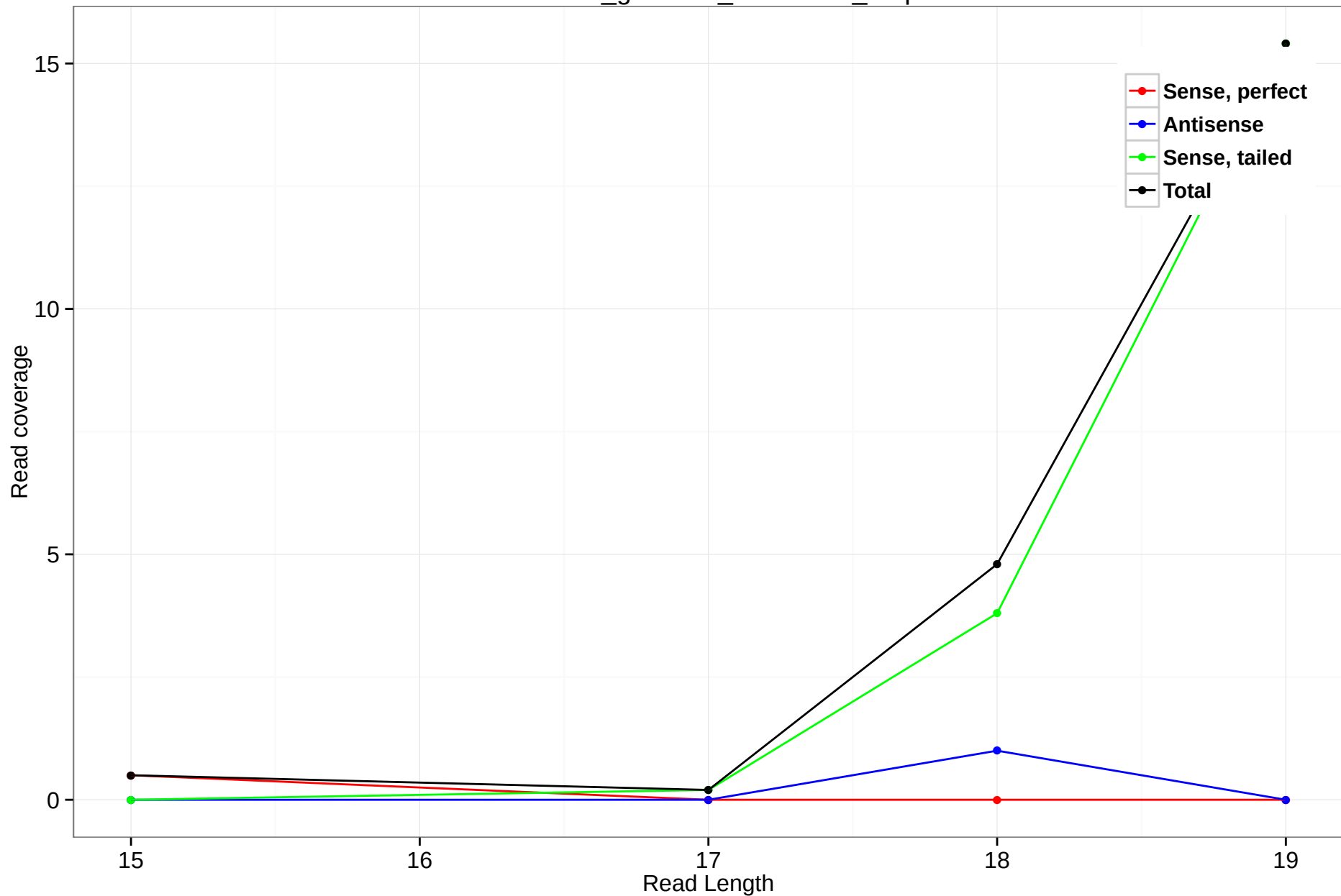
rheMac3_genscan_chr1.4533_3.3p
