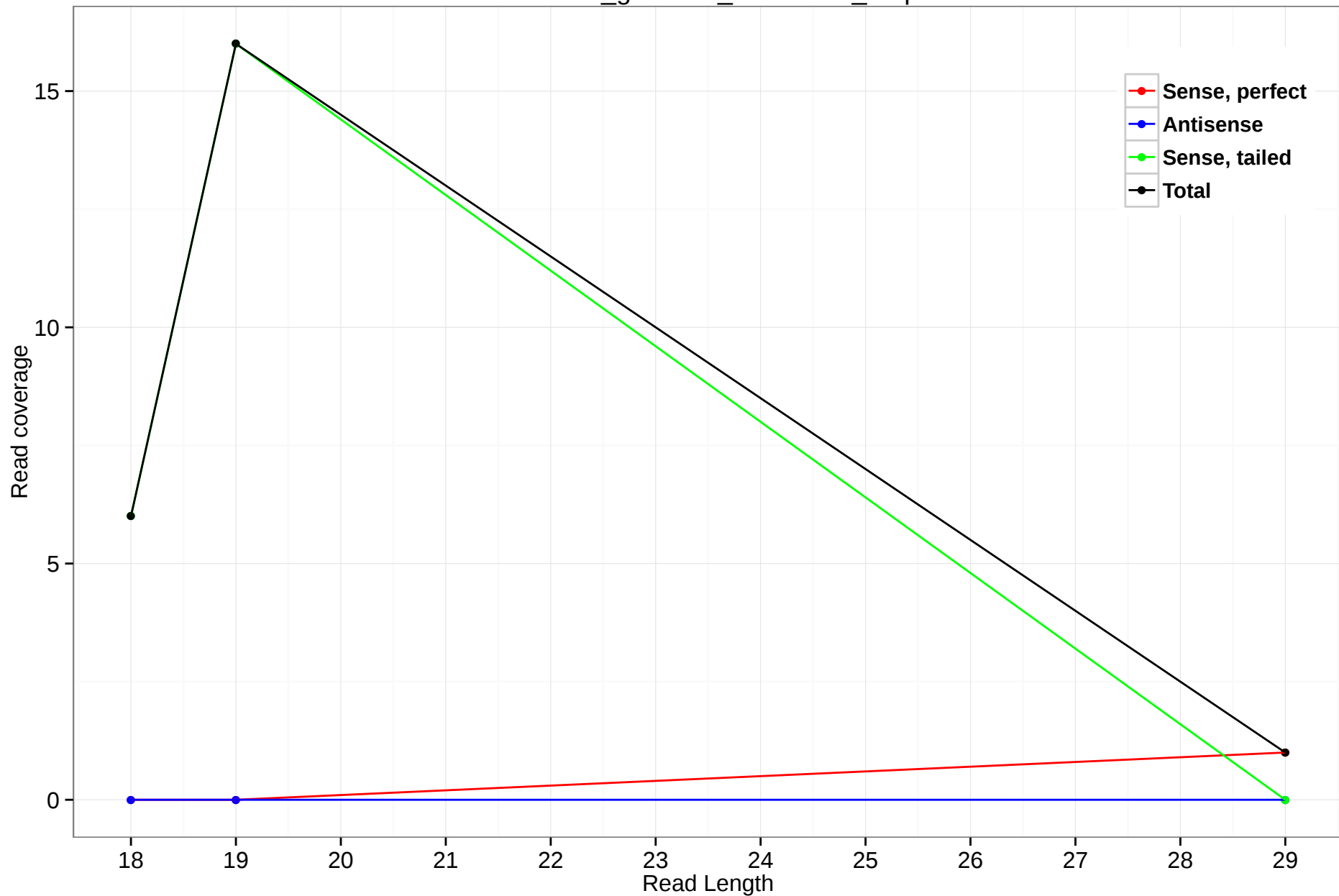
rheMac3_genscan_chr1.4382_3.3p
