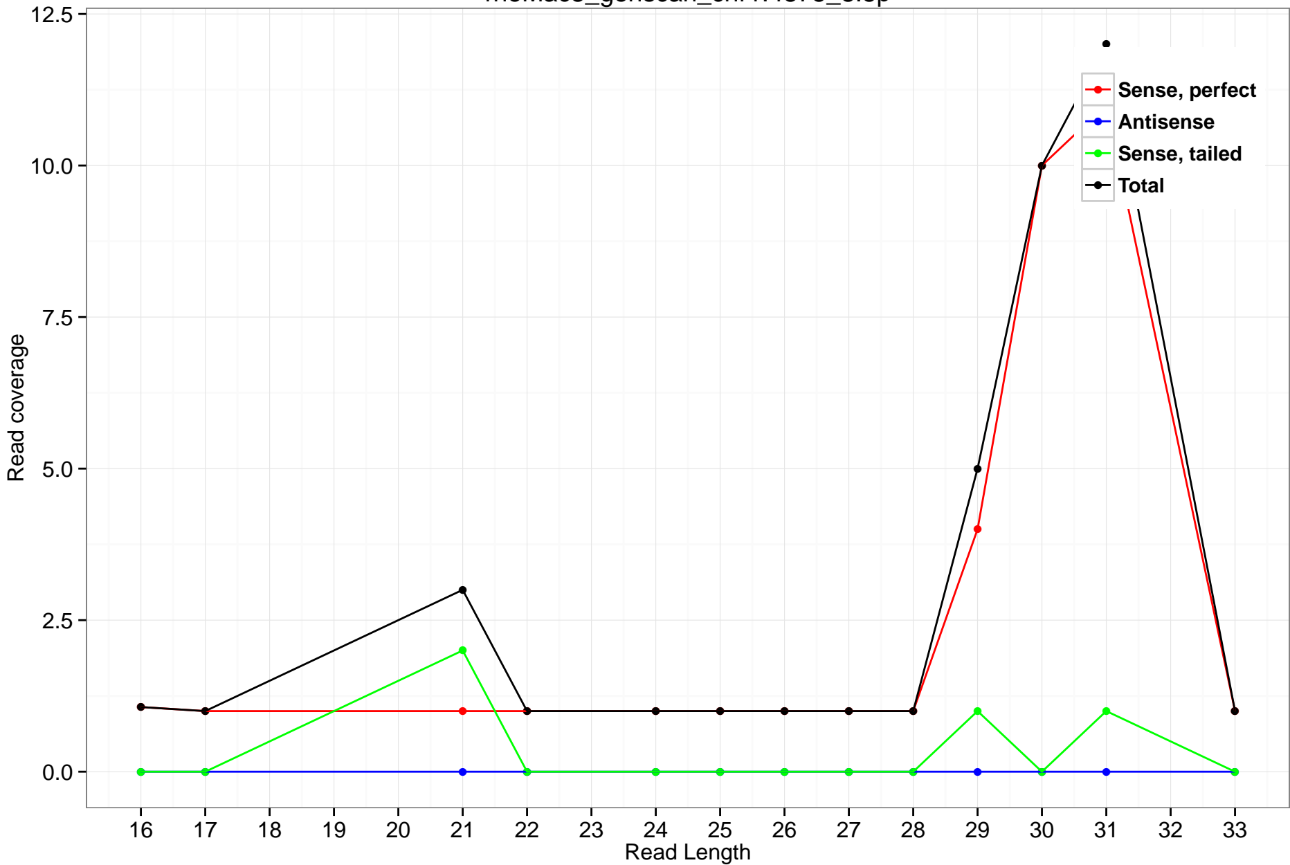
rheMac3_genscan_chr1.4375_8.5p
