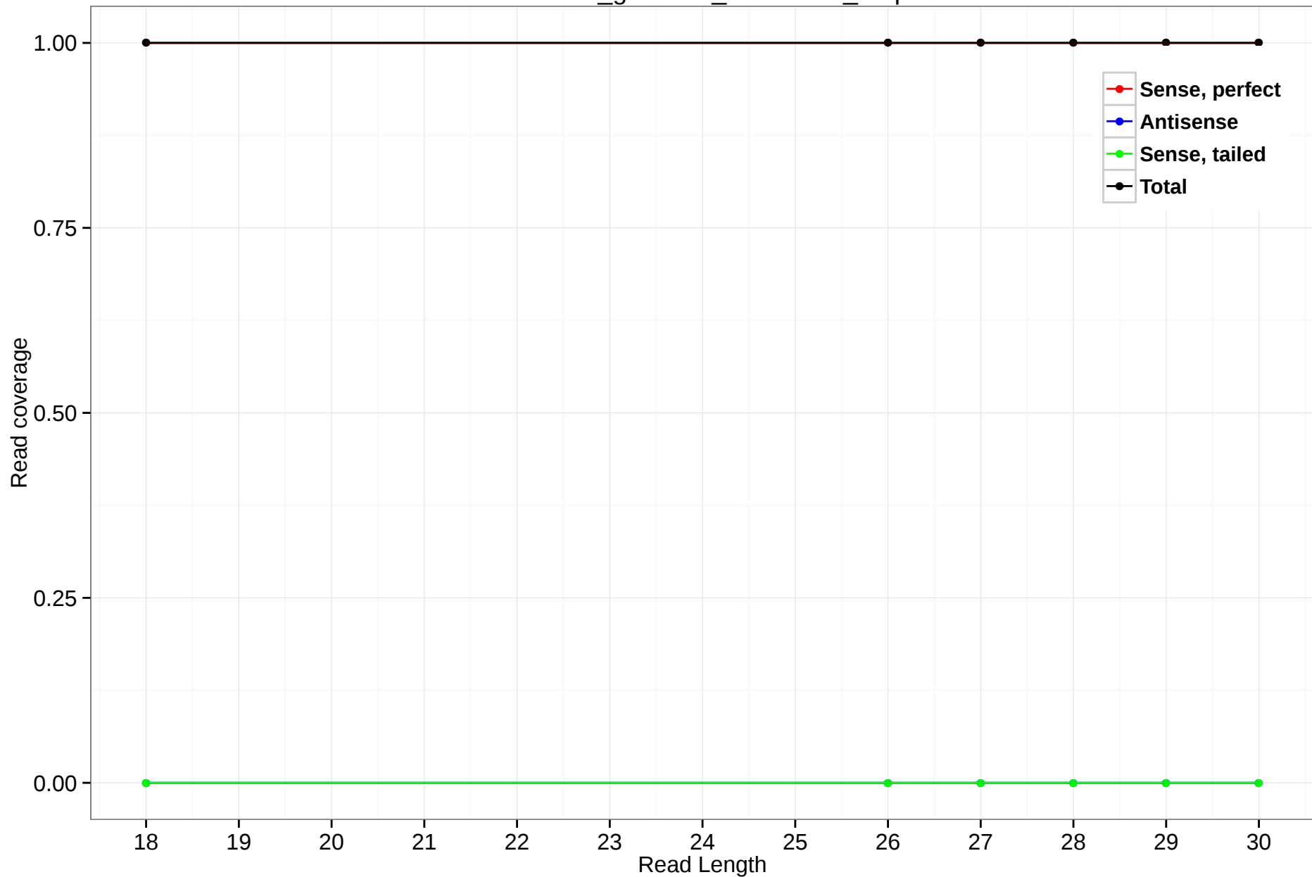
rheMac3_genscan_chr1.4371_4.5p
