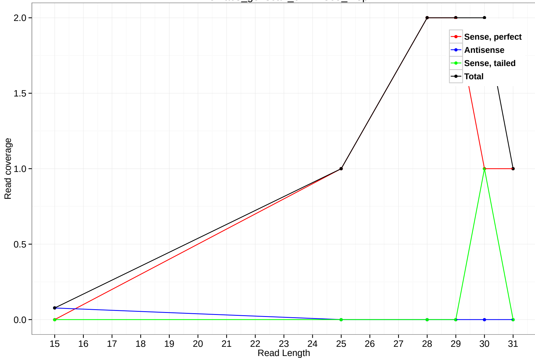
rheMac3_genscan_chr1.4369_4.3p
