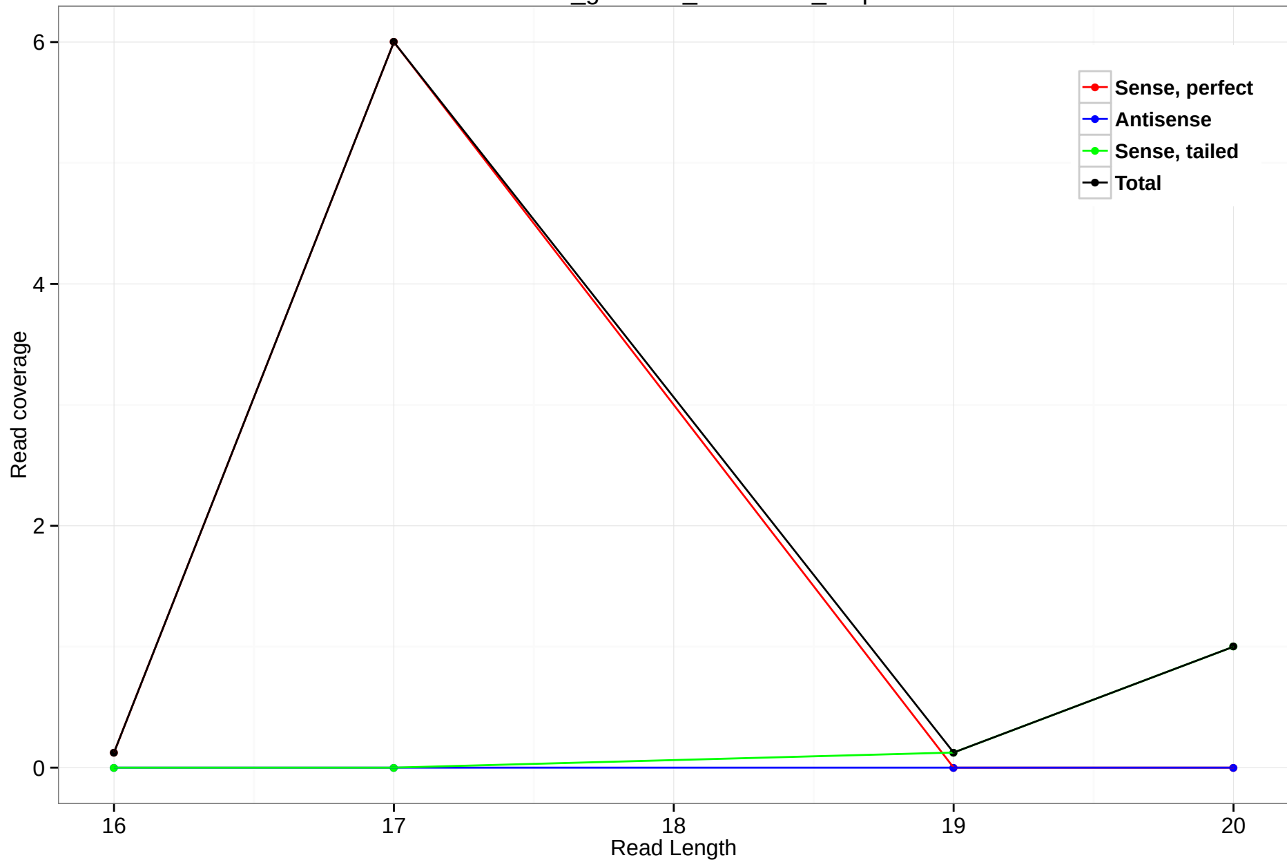
rheMac3_genscan_chr1.4171_9.3p
