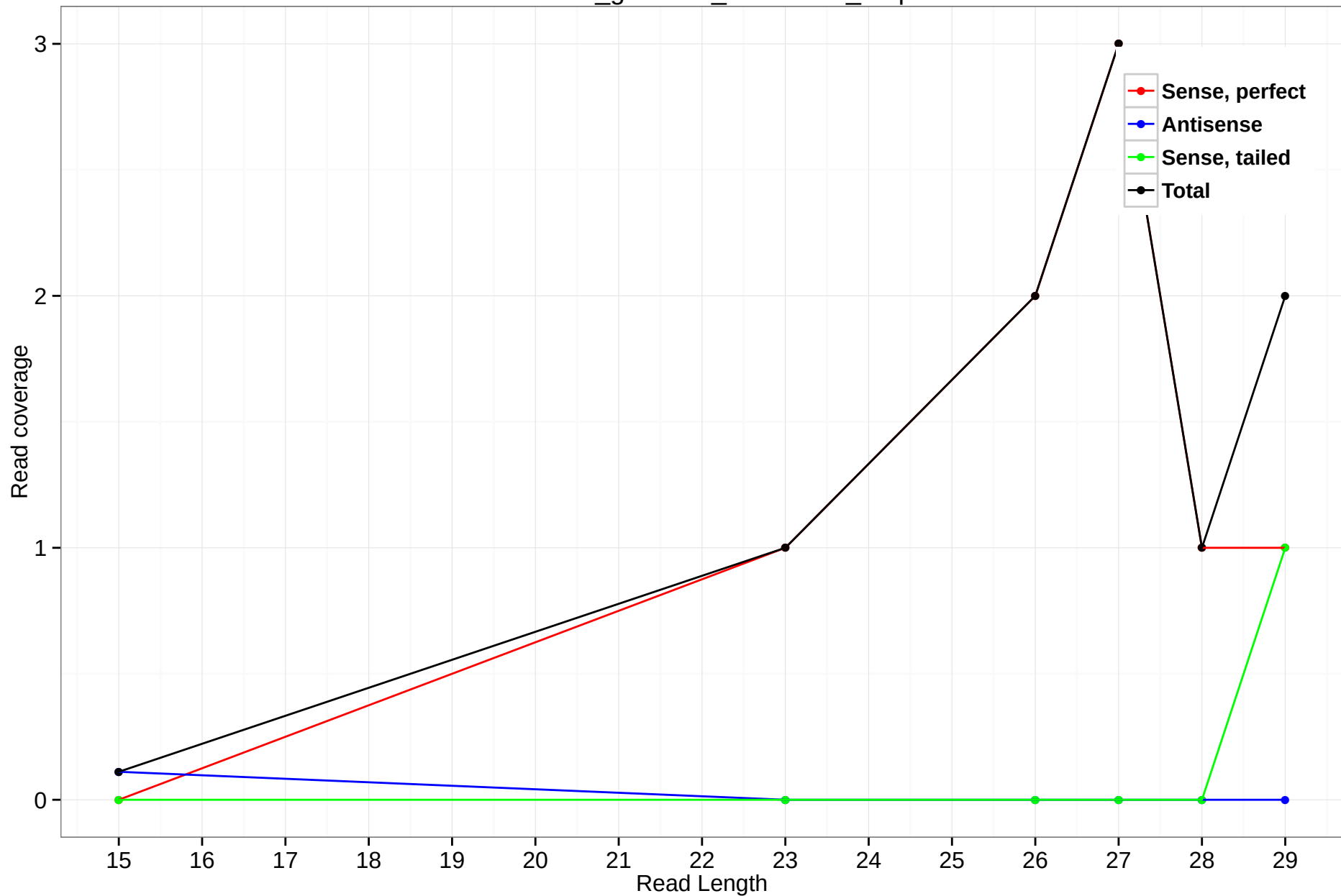
rheMac3_genscan_chr1.4082_2.3p
