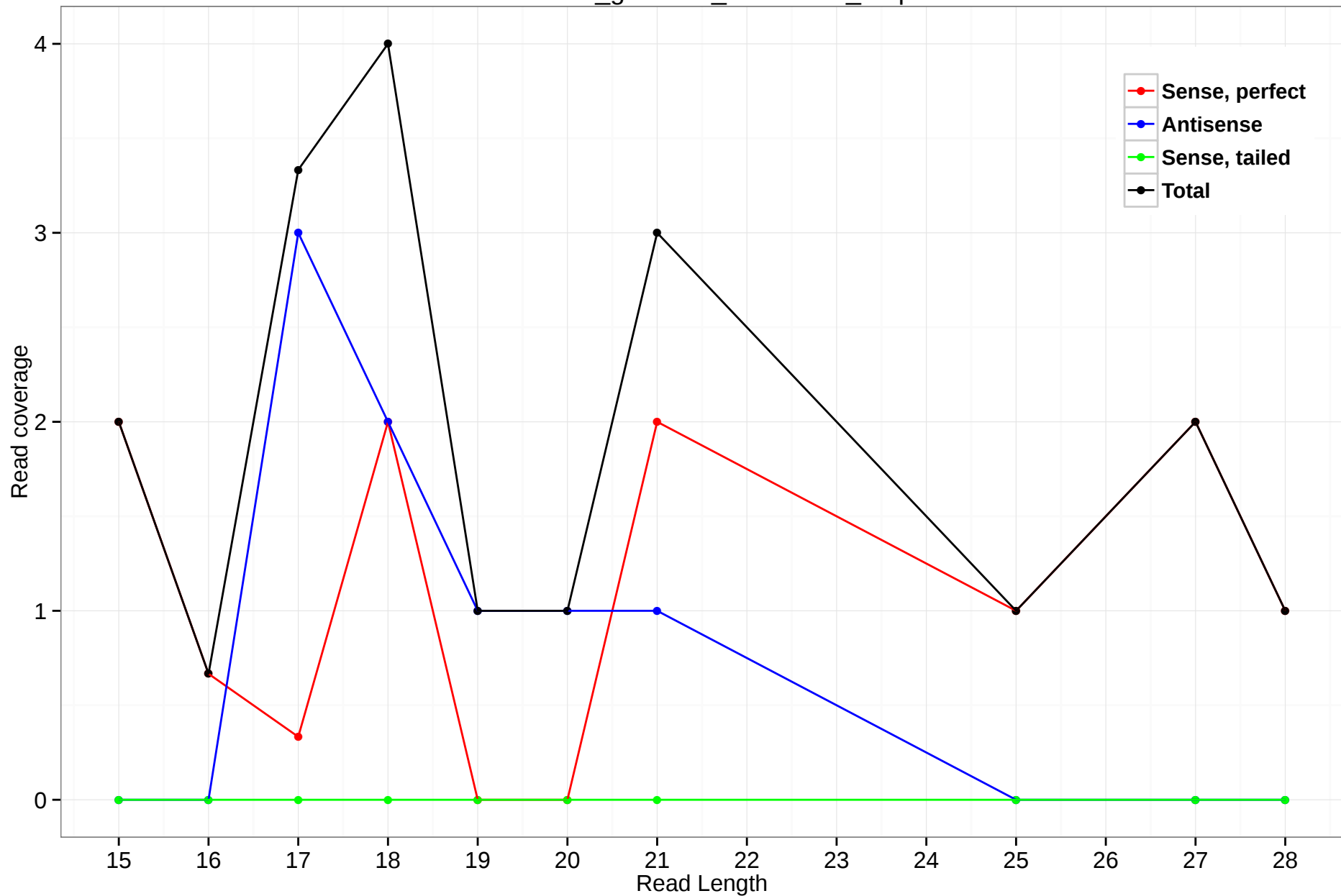
rheMac3_genscan_chr1.4062_3.3p
