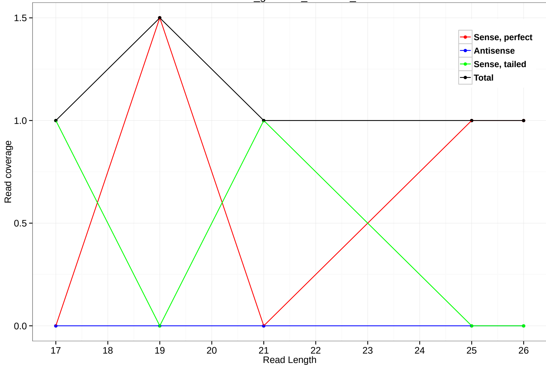
rheMac3_genscan_chr1.404_10
