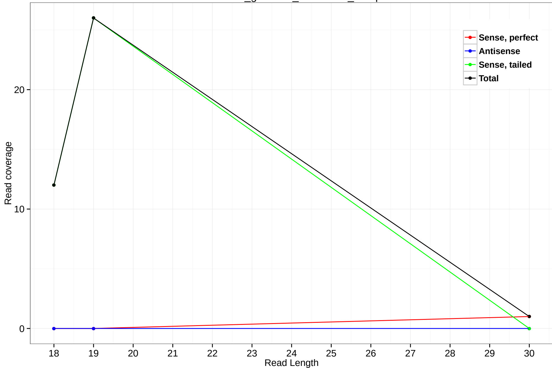
rheMac3_genscan_chr1.4035_10.5p
