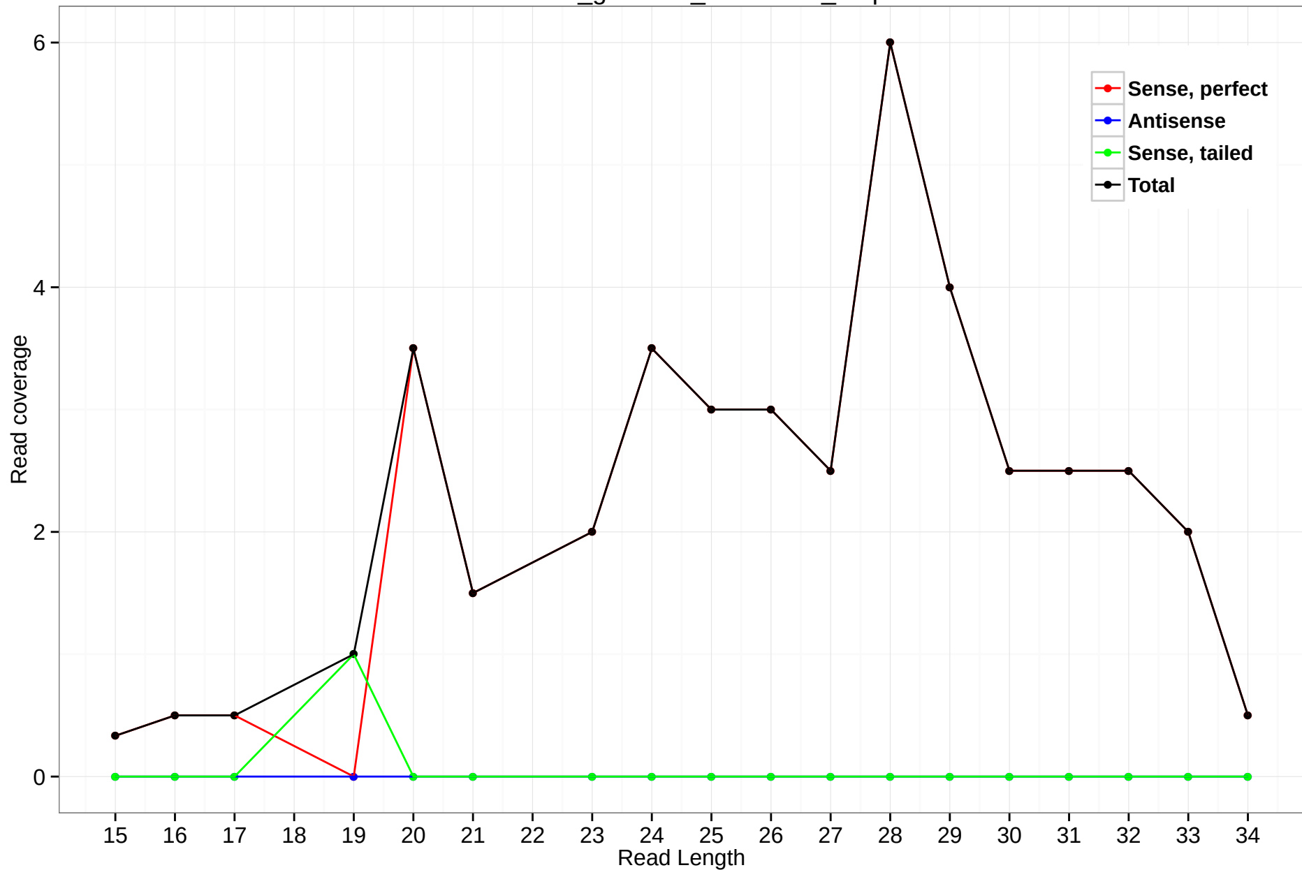
rheMac3_genscan_chr1.4027_9.5p
