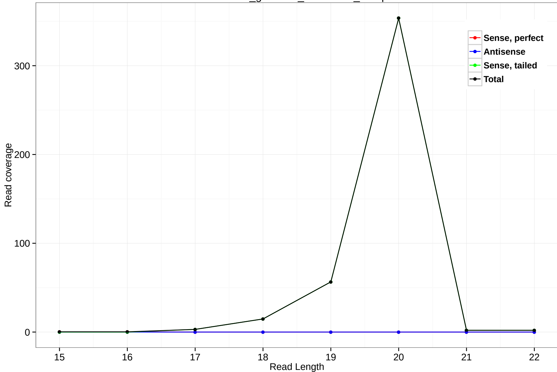
rheMac3_genscan_chr1.4002_25.5p
