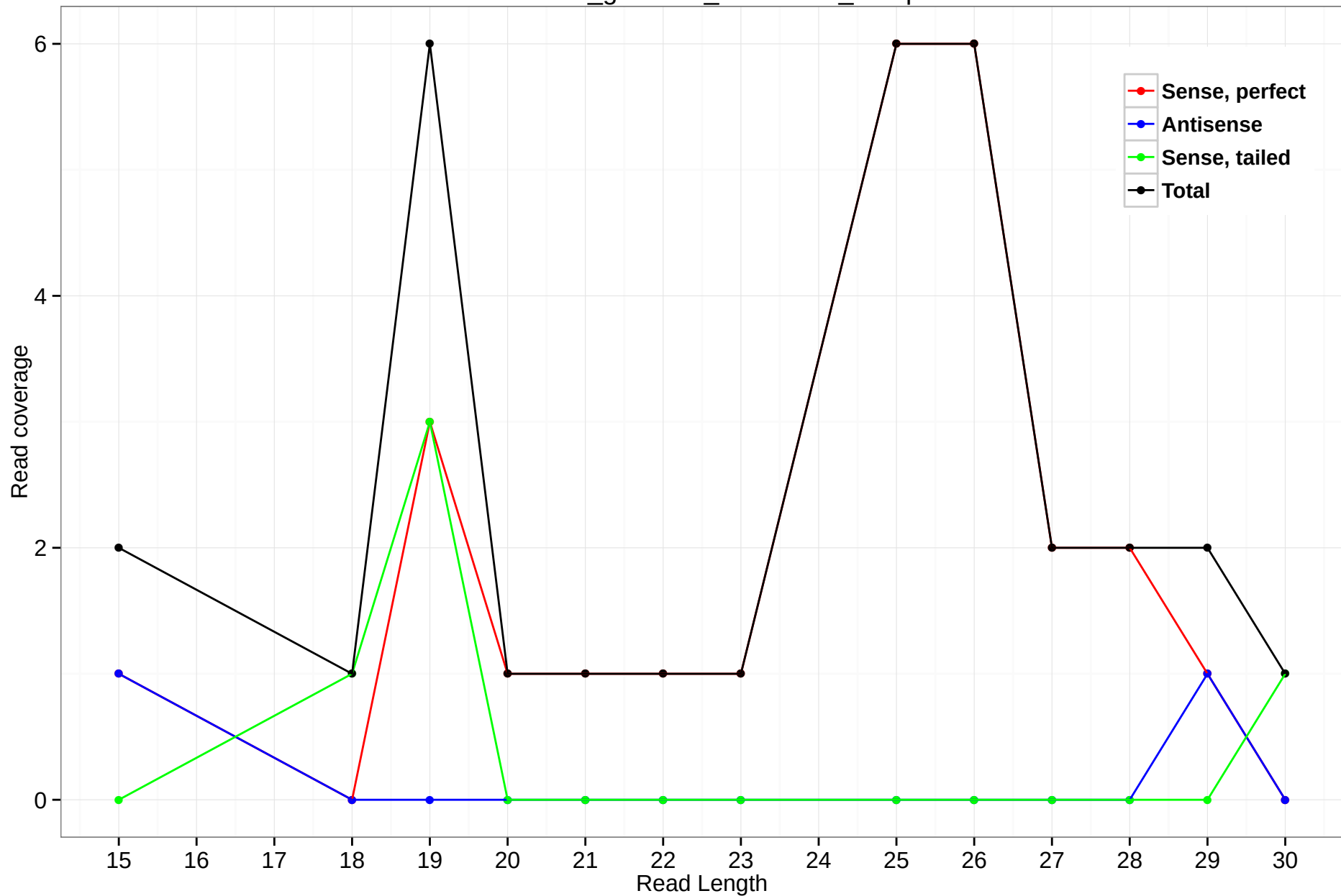
rheMac3_genscan_chr1.3970_11.5p
