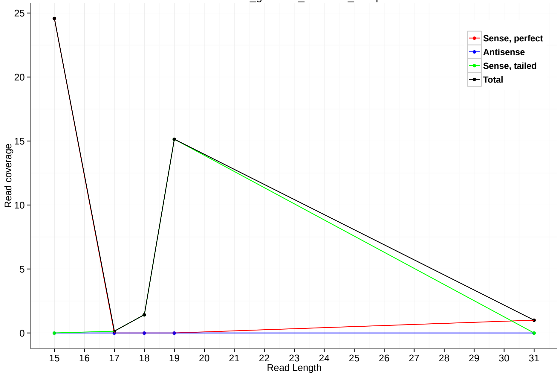
rheMac3_genscan_chr1.396_19.5p
