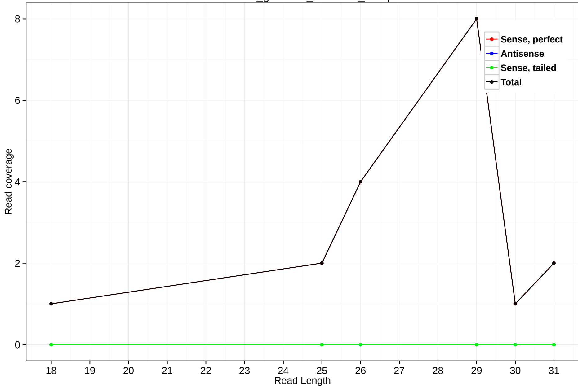
rheMac3_genscan_chr1.396_17.3p
