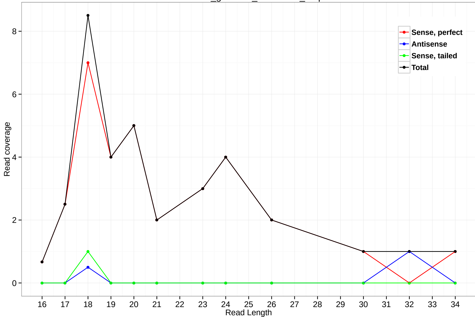
rheMac3_genscan_chr1.3956_0.3p
