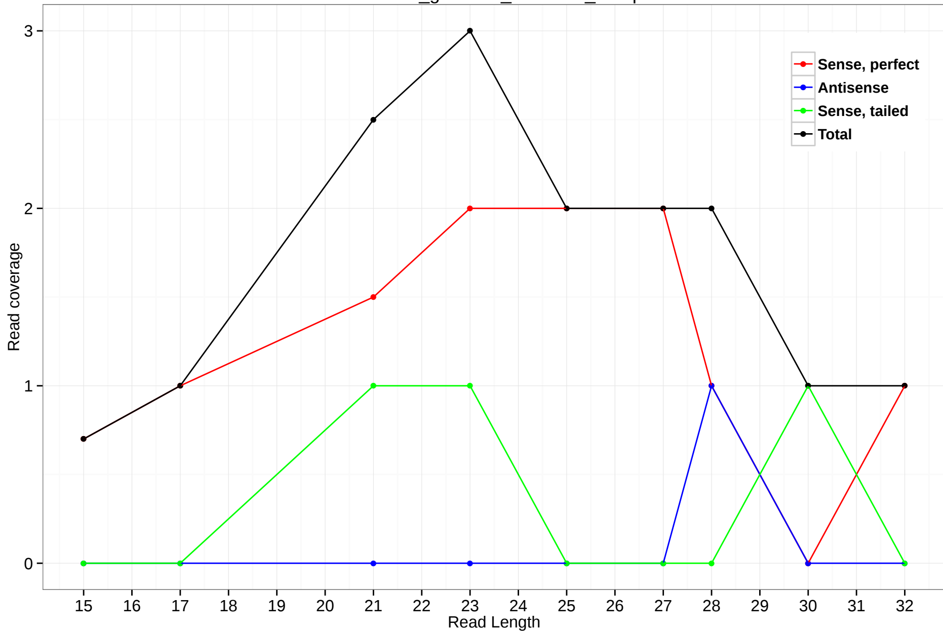
rheMac3_genscan_chr1.392_10.5p
