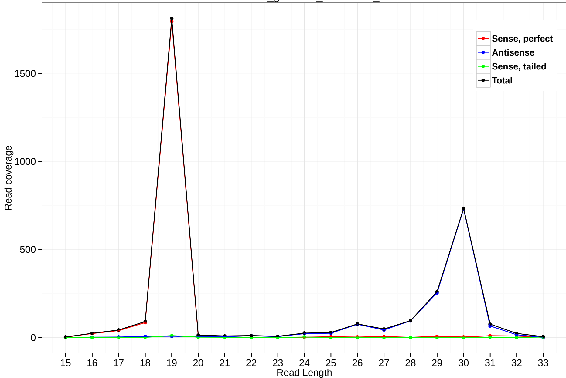
rheMac3_genscan_chr1.3881_3
