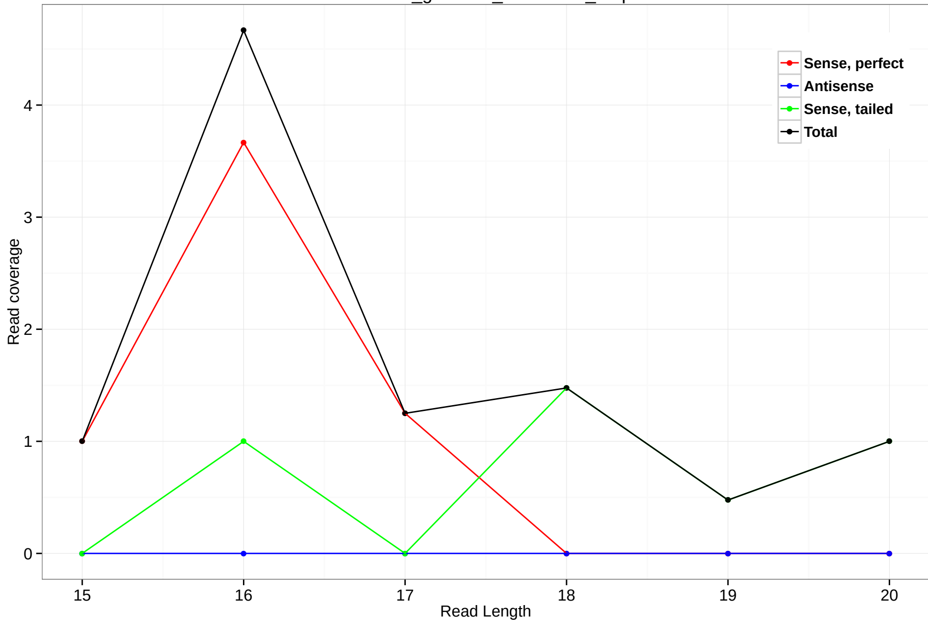
rheMac3_genscan_chr1.3872_5.5p
