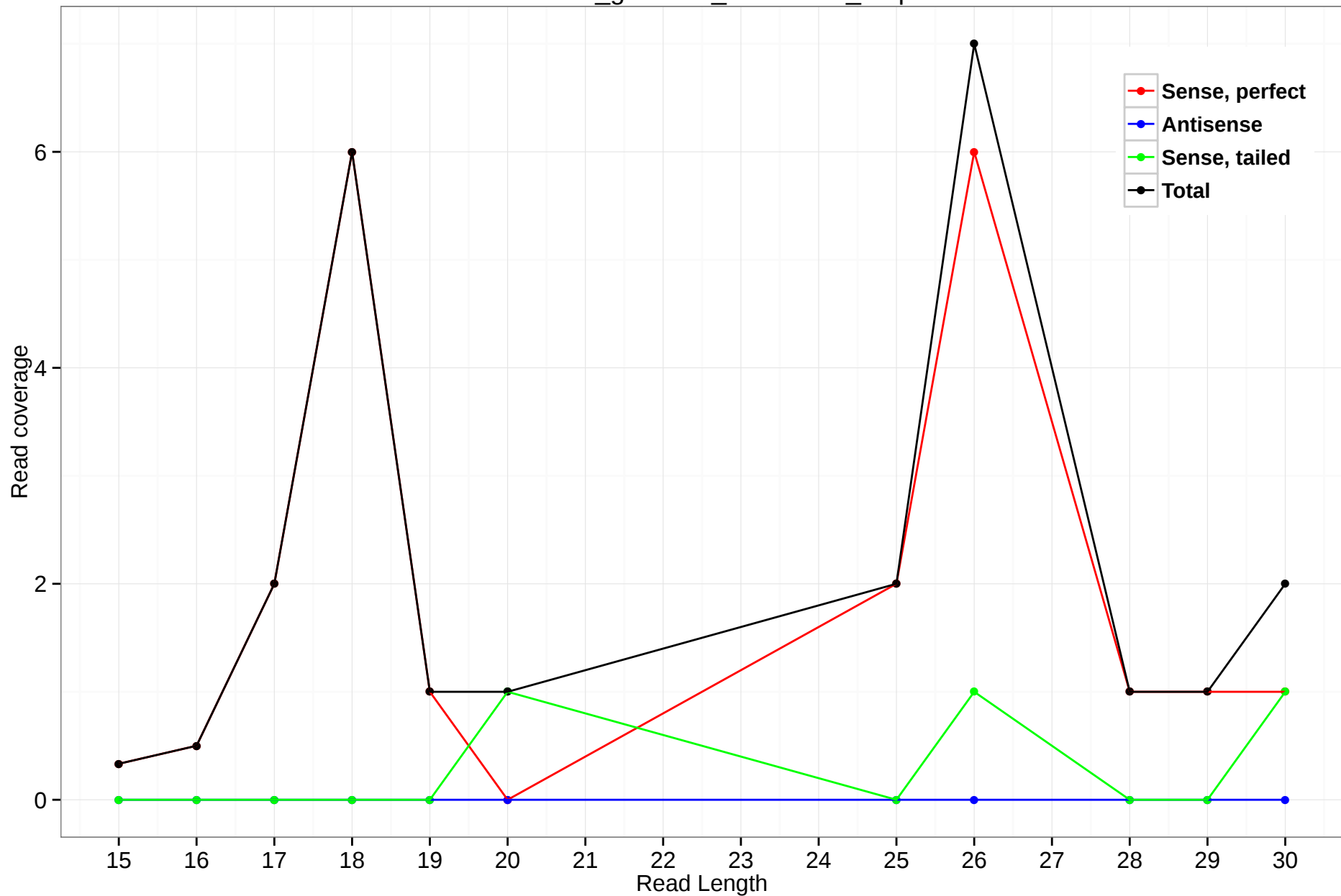
rheMac3_genscan_chr1.3870_3.3p
