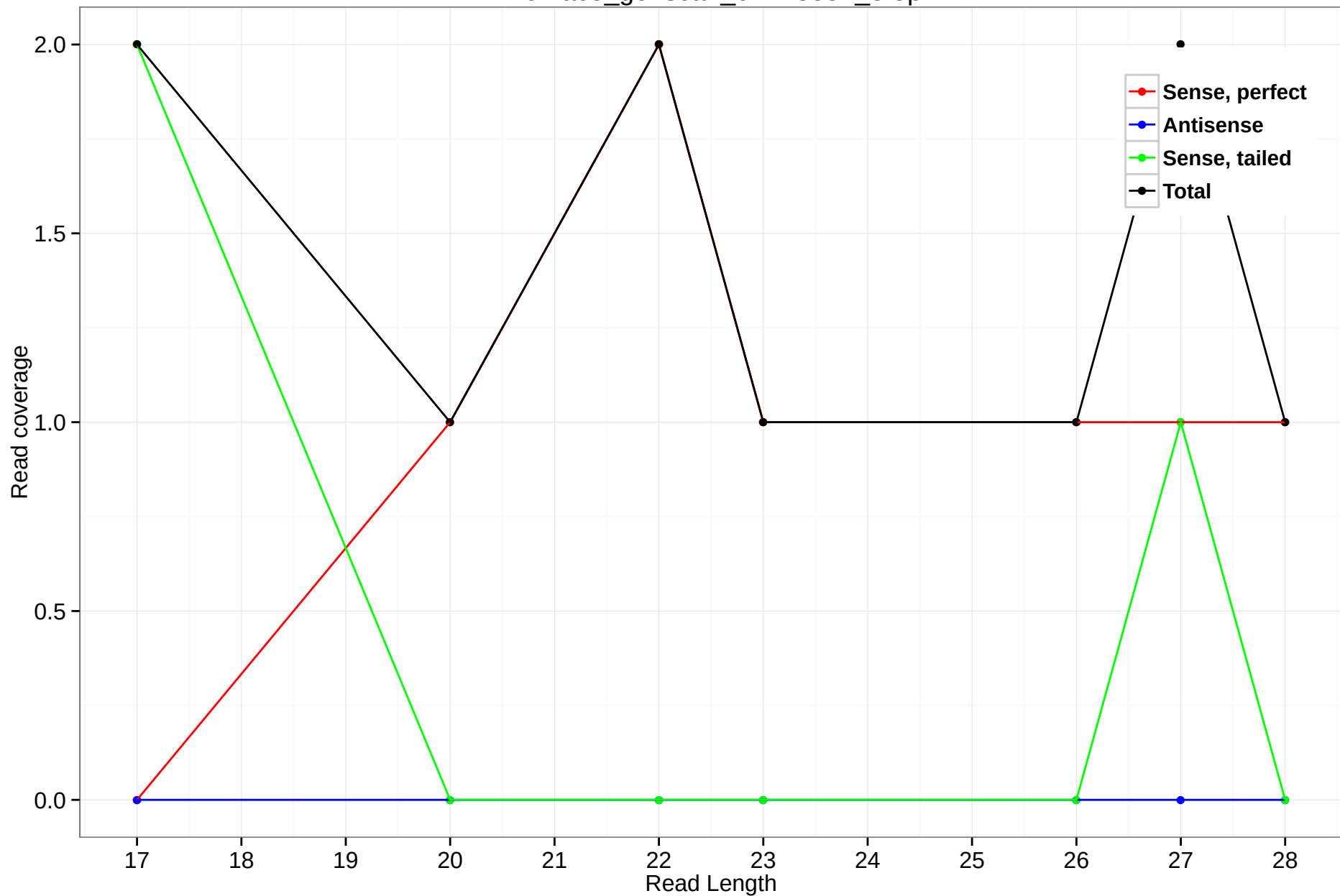
rheMac3_genscan_chr1.3851_3.5p
