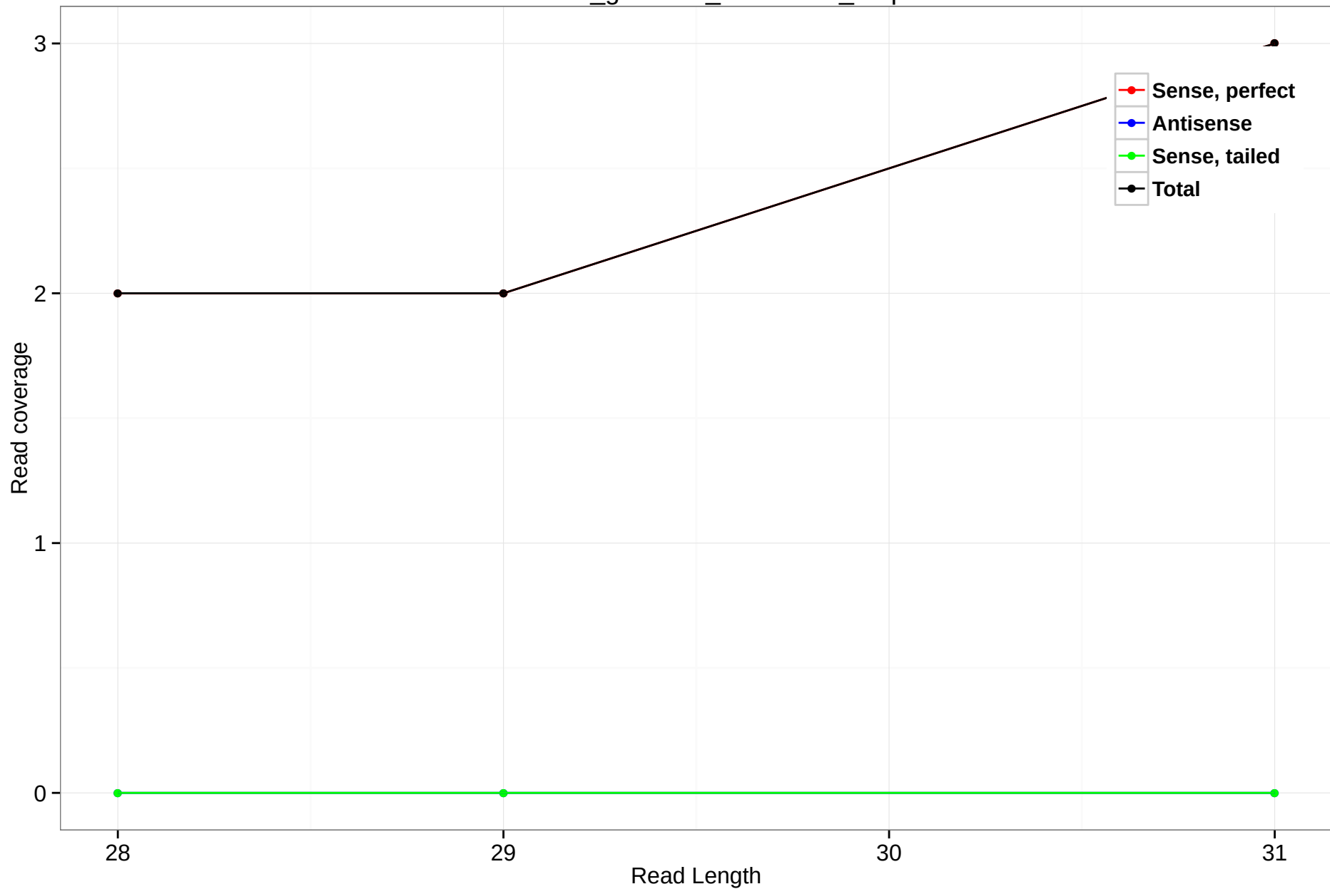
rheMac3_genscan_chr1.3851_0.5p
