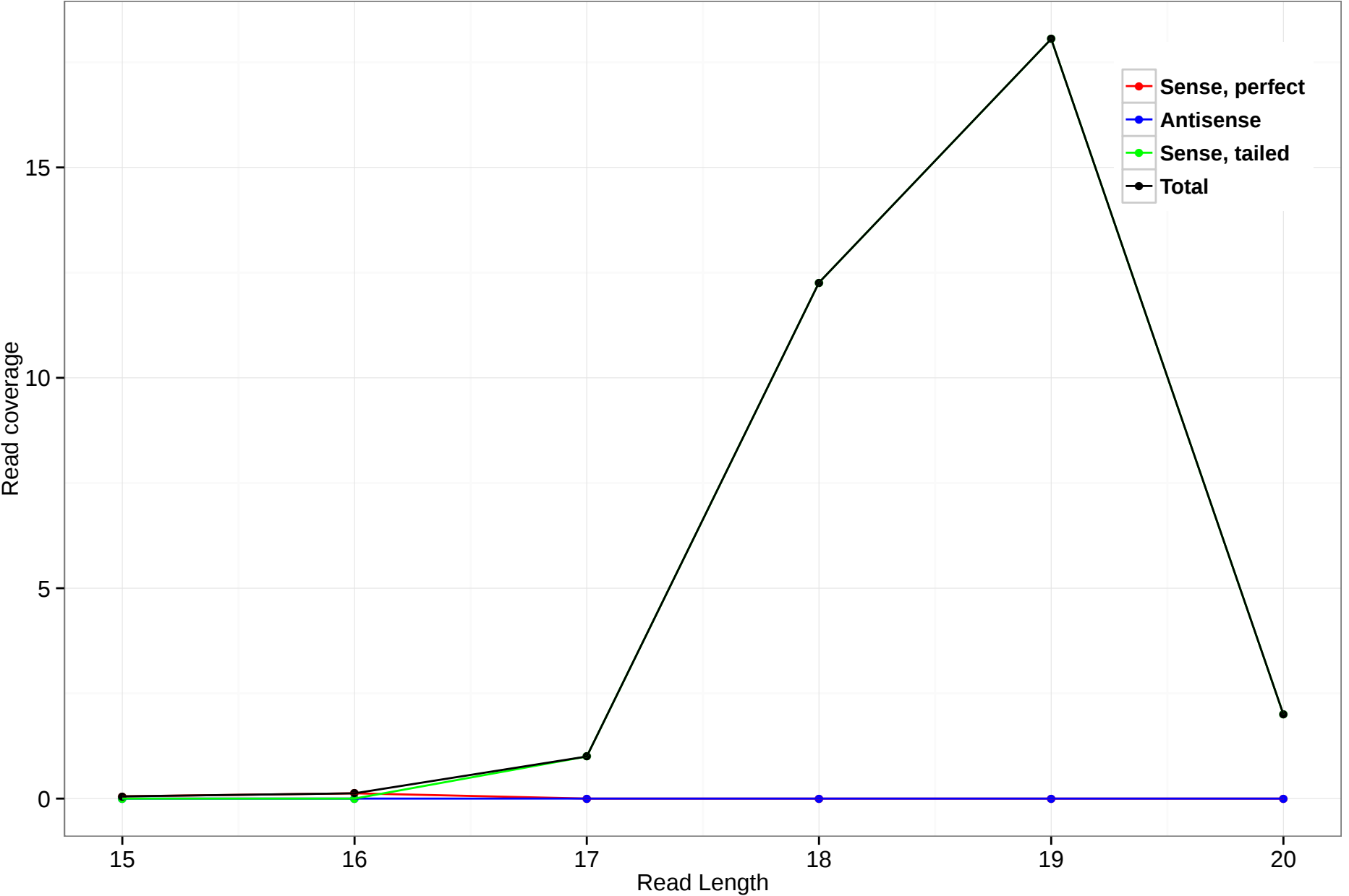
rheMac3_genscan_chr1.3800_16
