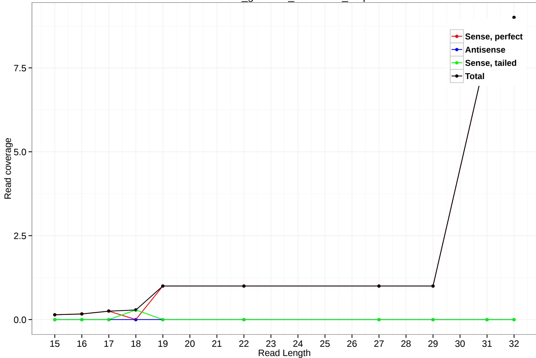
rheMac3_genscan_chr1.3798_3.5p
