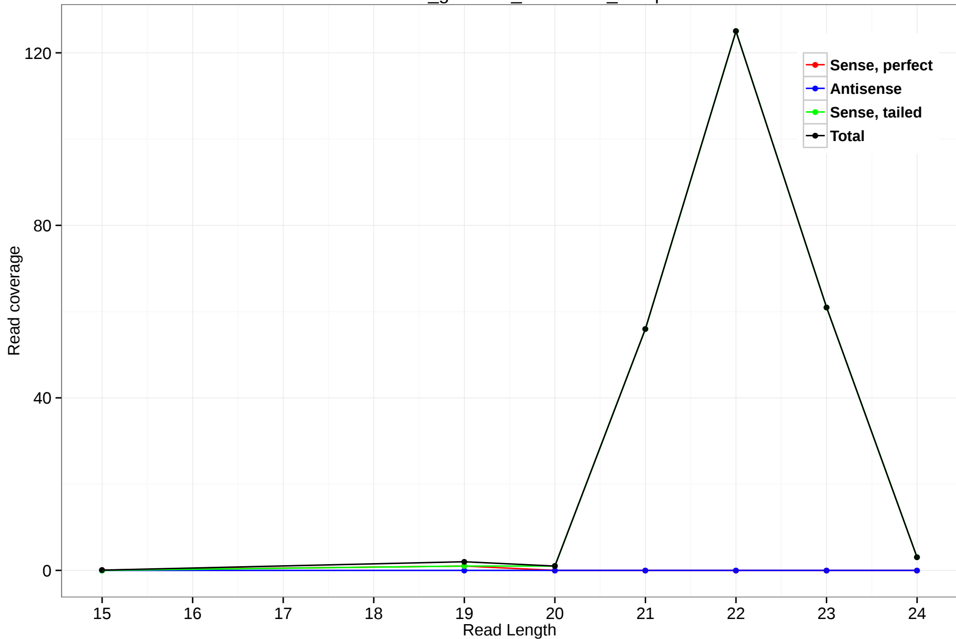
rheMac3_genscan_chr1.3761_45.5p
