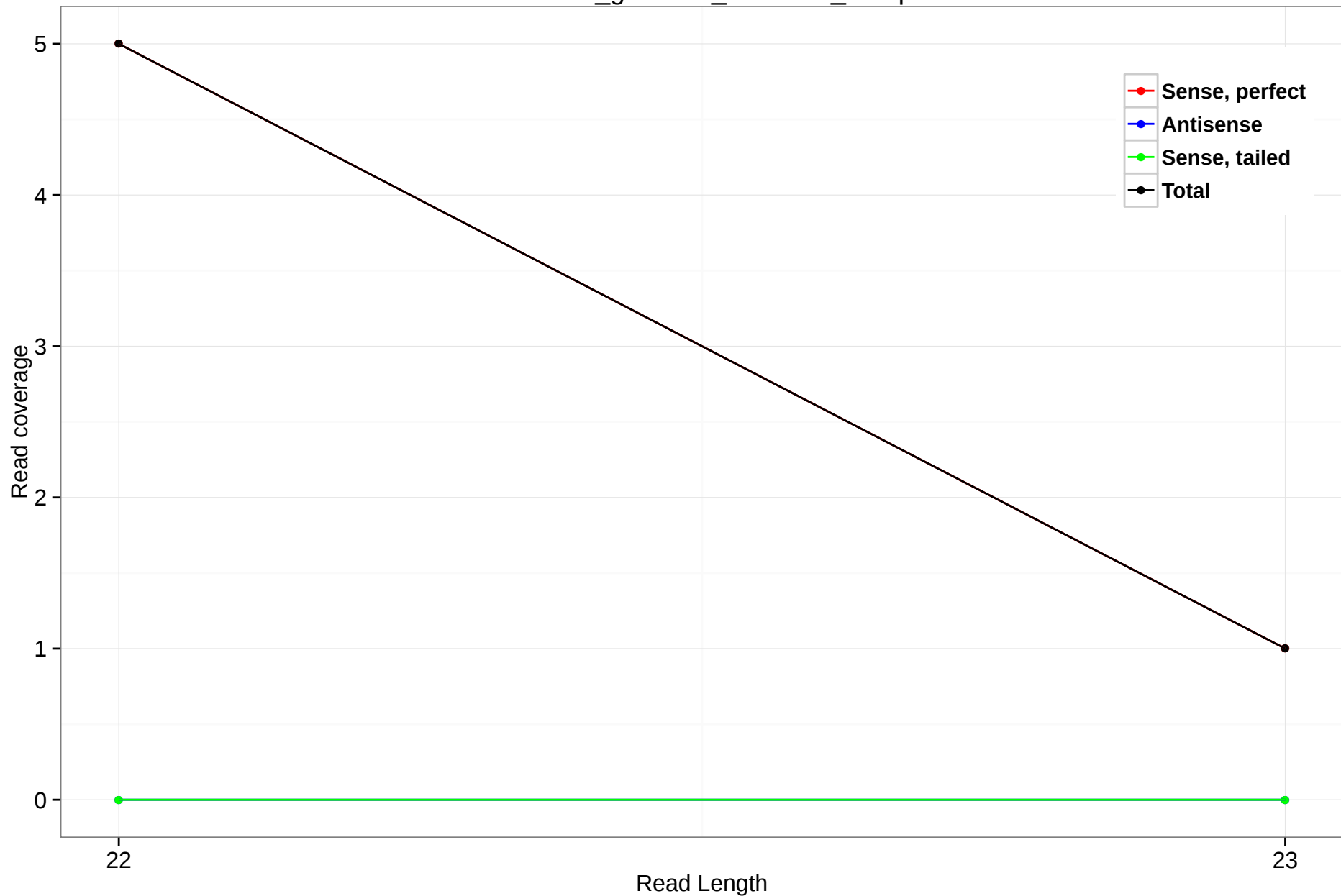
rheMac3_genscan_chr1.371_46.3p
