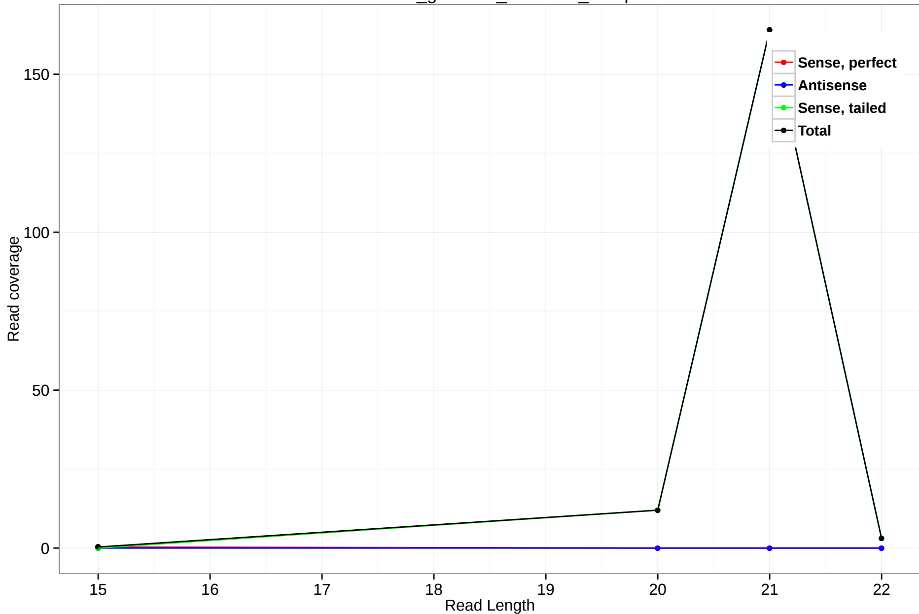
rheMac3_genscan_chr1.371_12.5p
