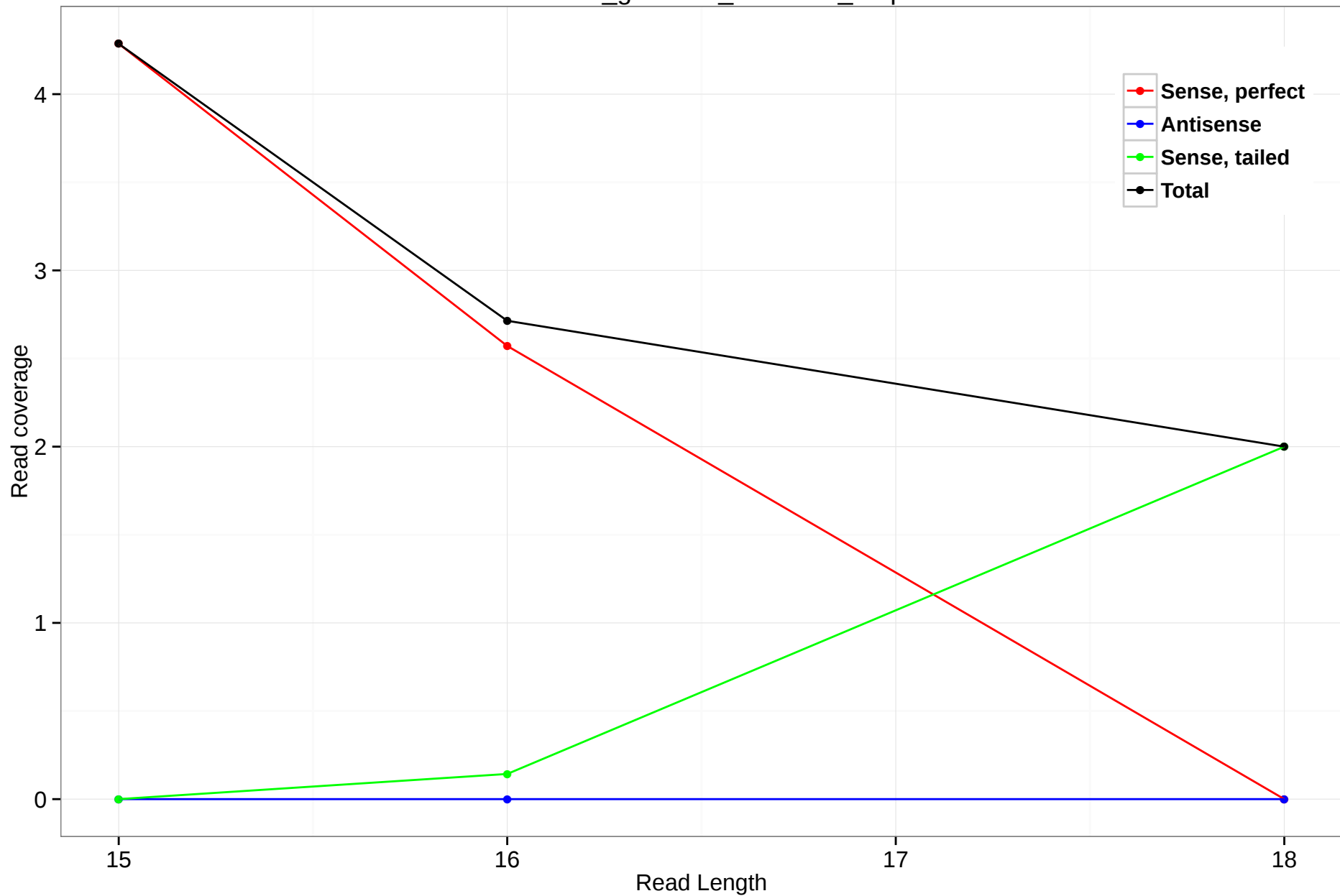
rheMac3_genscan_chr1.366_4.5p
