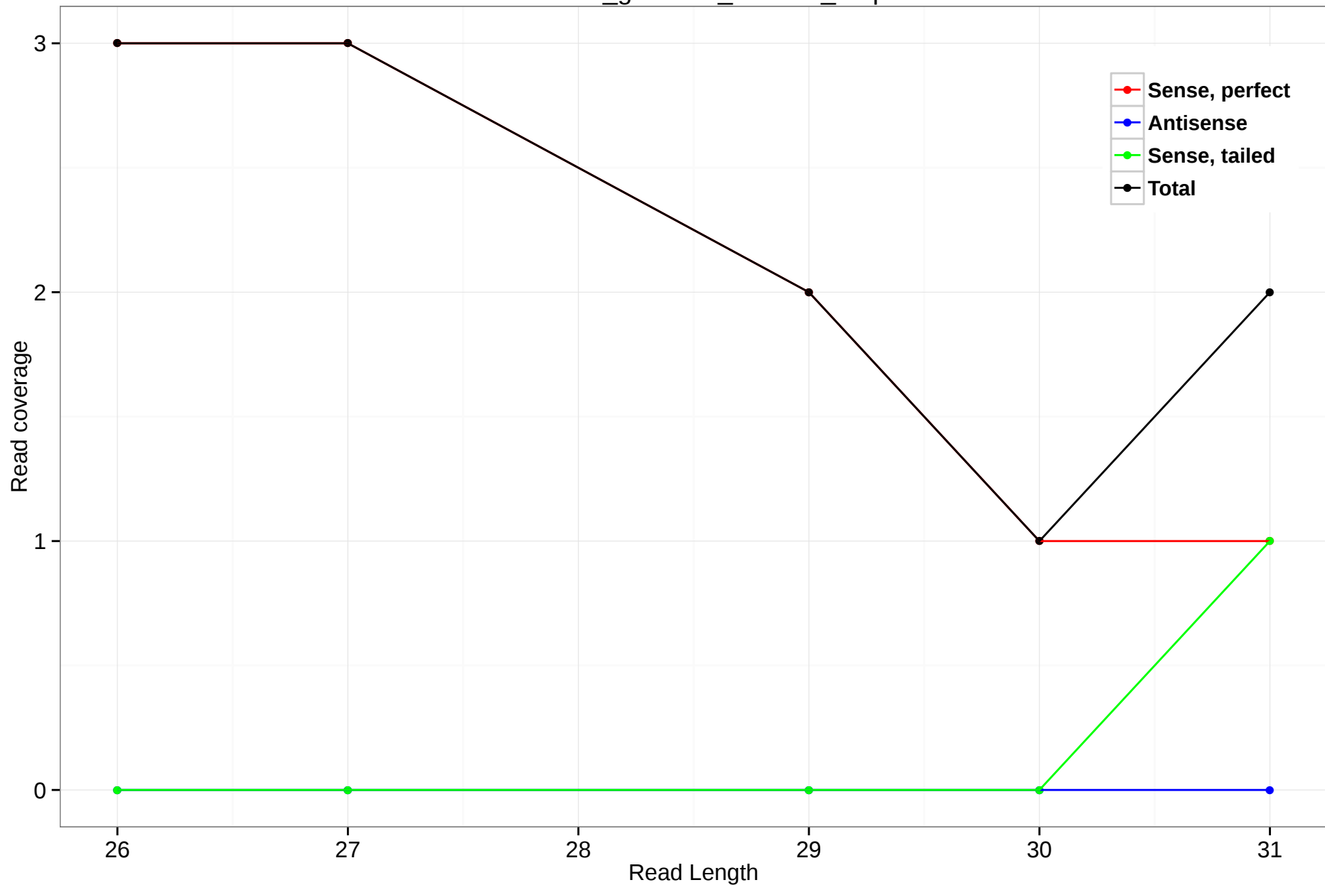
rheMac3_genscan_chr1.35_0.5p
