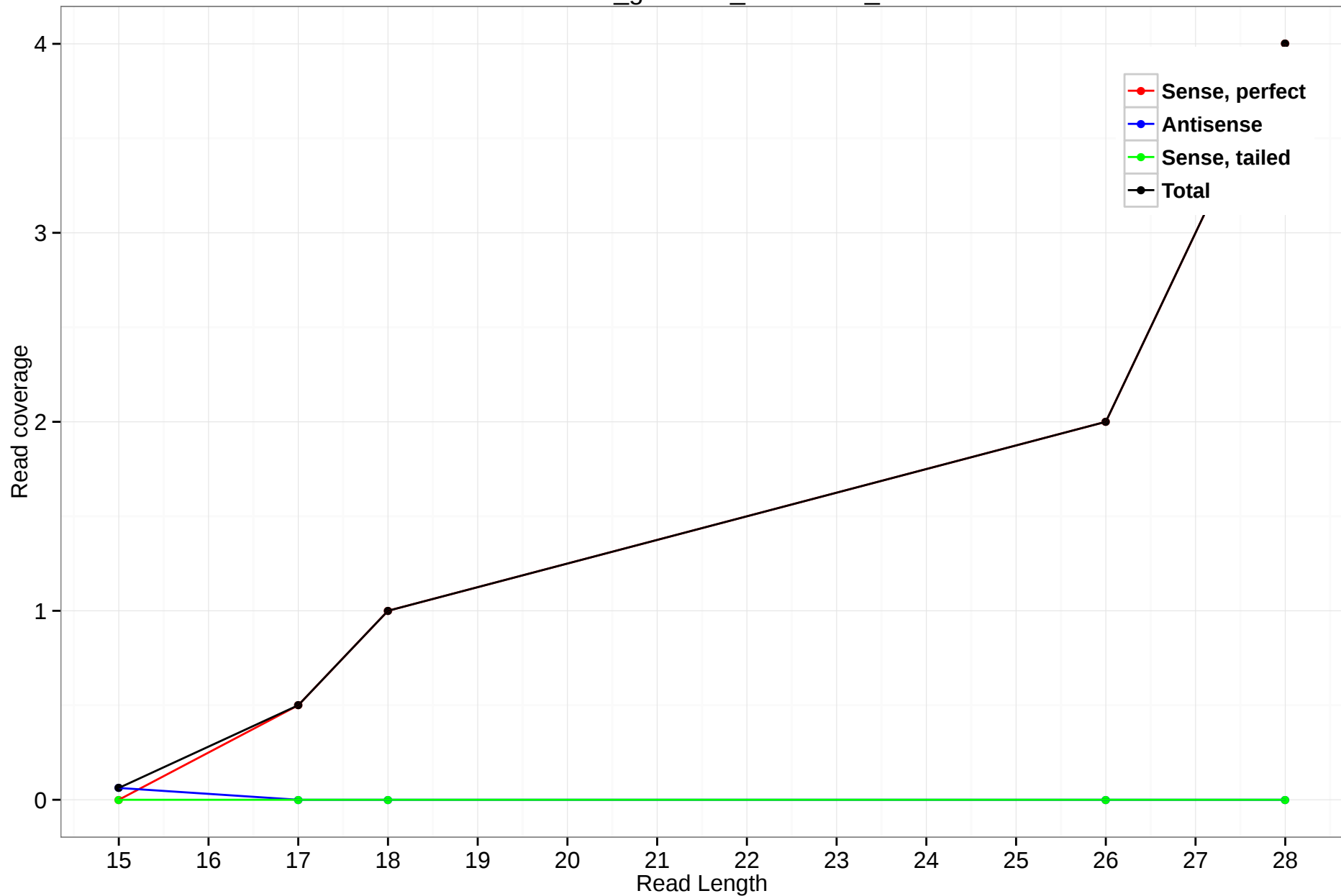
rheMac3_genscan_chr1.3590_0
