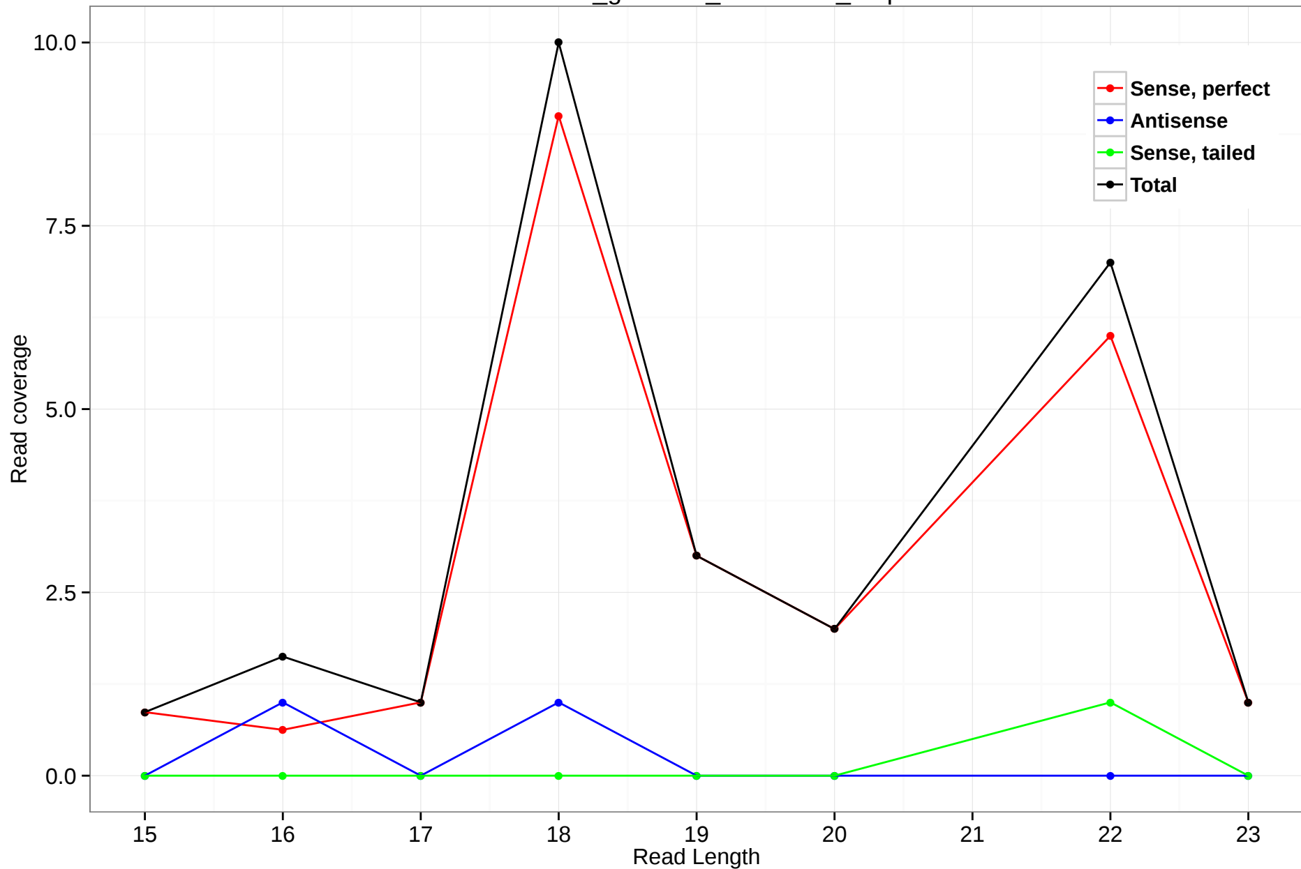
rheMac3_genscan_chr1.3560_0.3p
