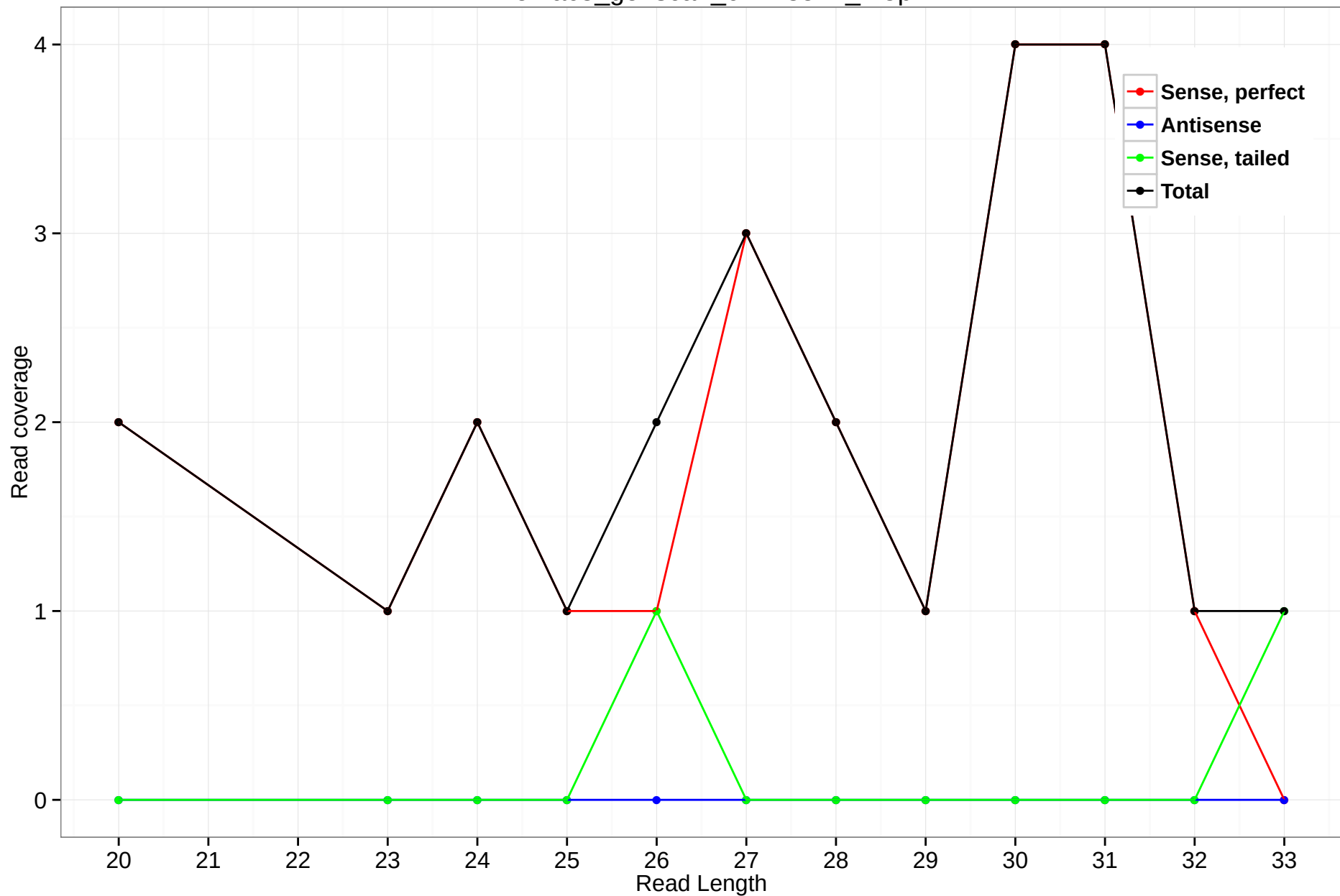
rheMac3_genscan_chr1.3514_4.5p
