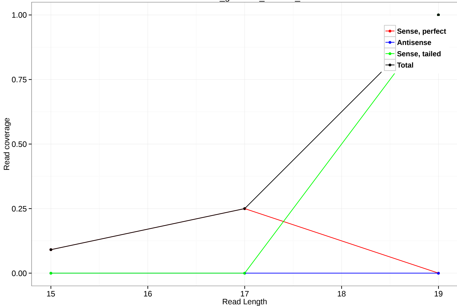
rheMac3_genscan_chr1.34_9
