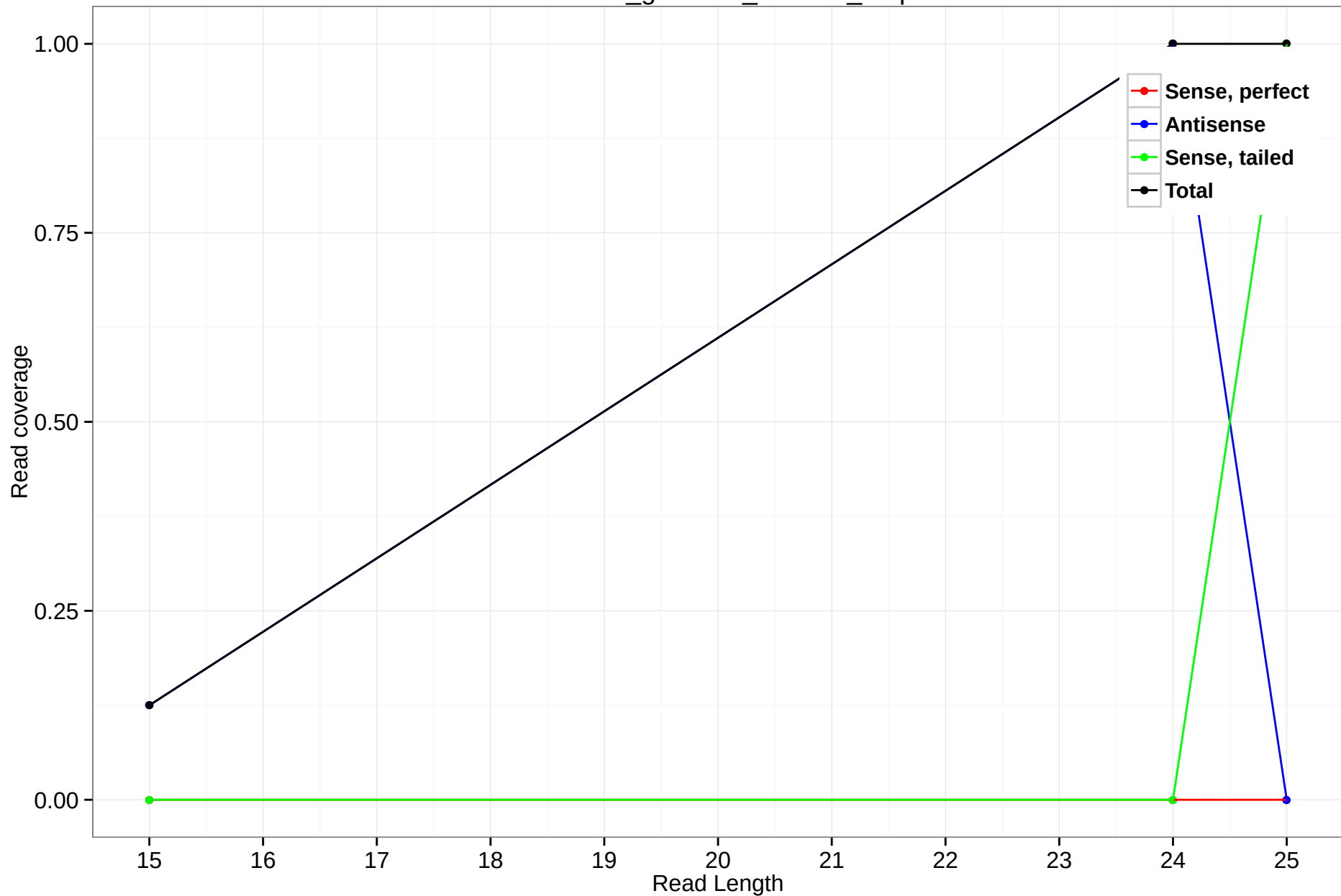
rheMac3_genscan_chr1.34_3.3p
