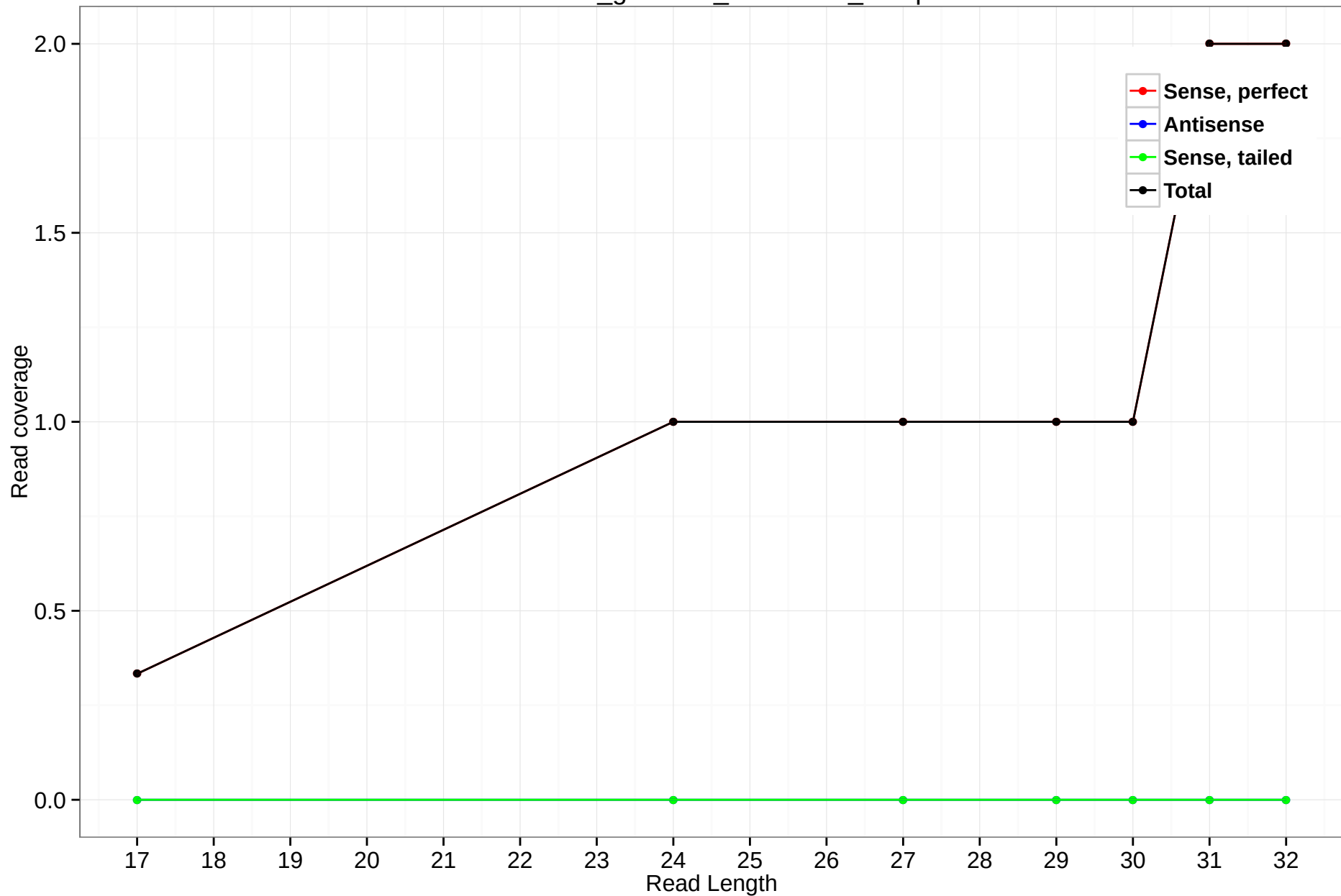
rheMac3_genscan_chr1.3499_11.5p
