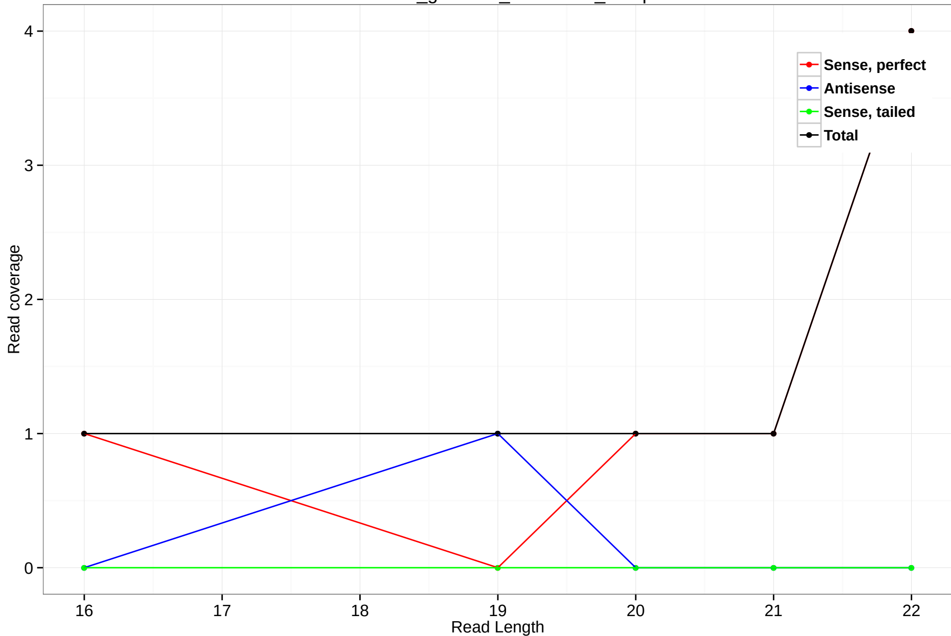
rheMac3_genscan_chr1.3494_26.3p
