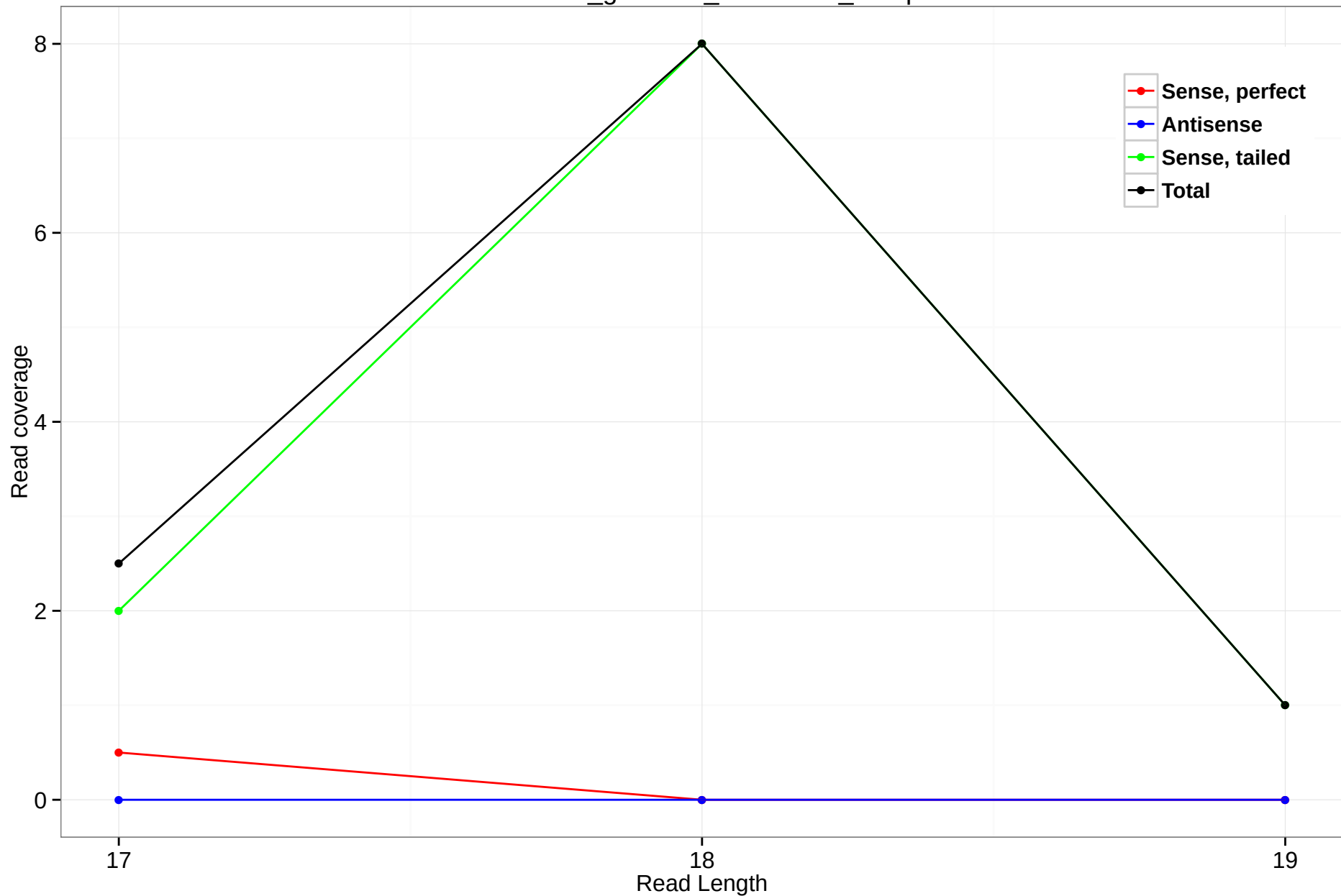
rheMac3_genscan_chr1.3494_10.3p
