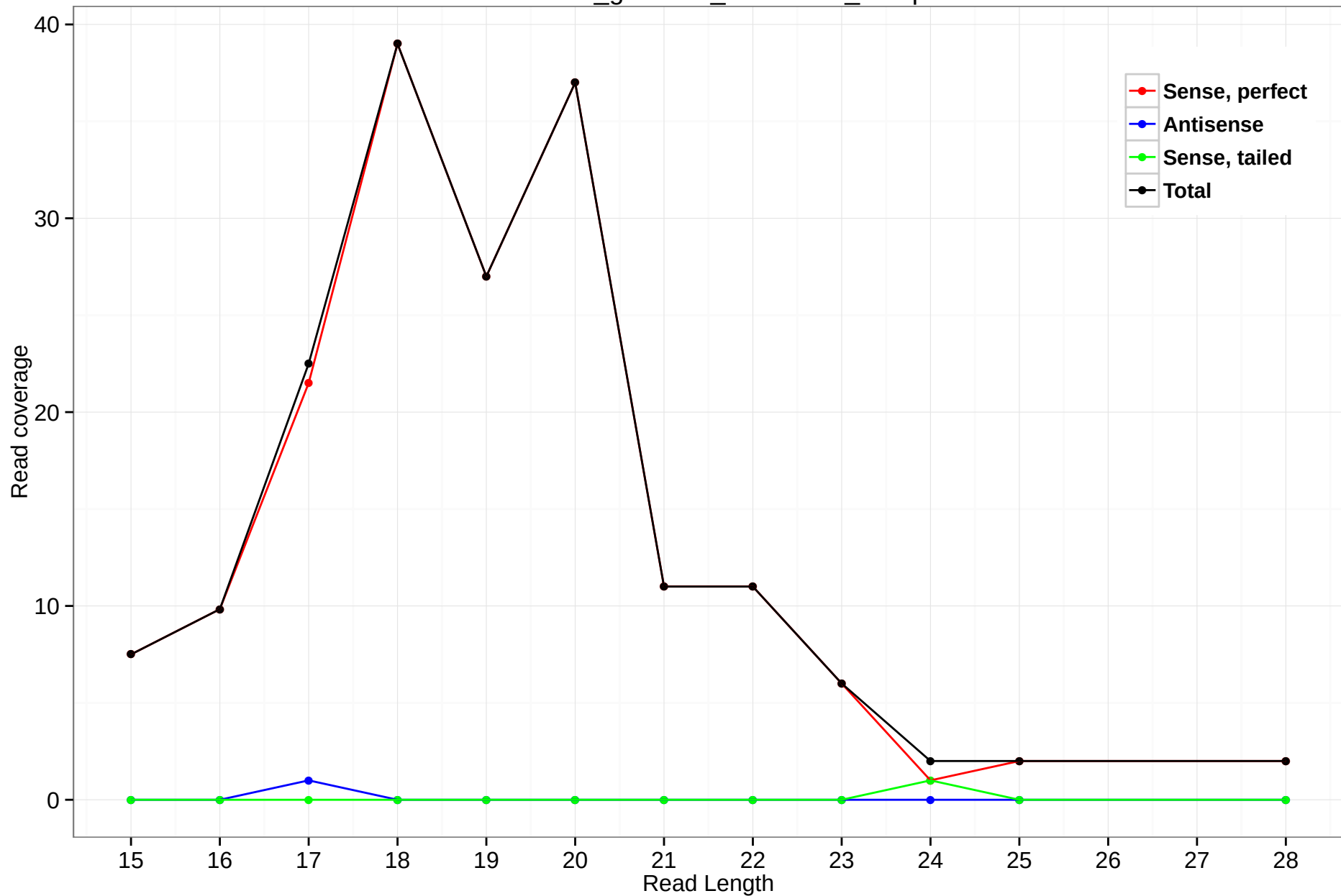
rheMac3_genscan_chr1.3439_19.5p
