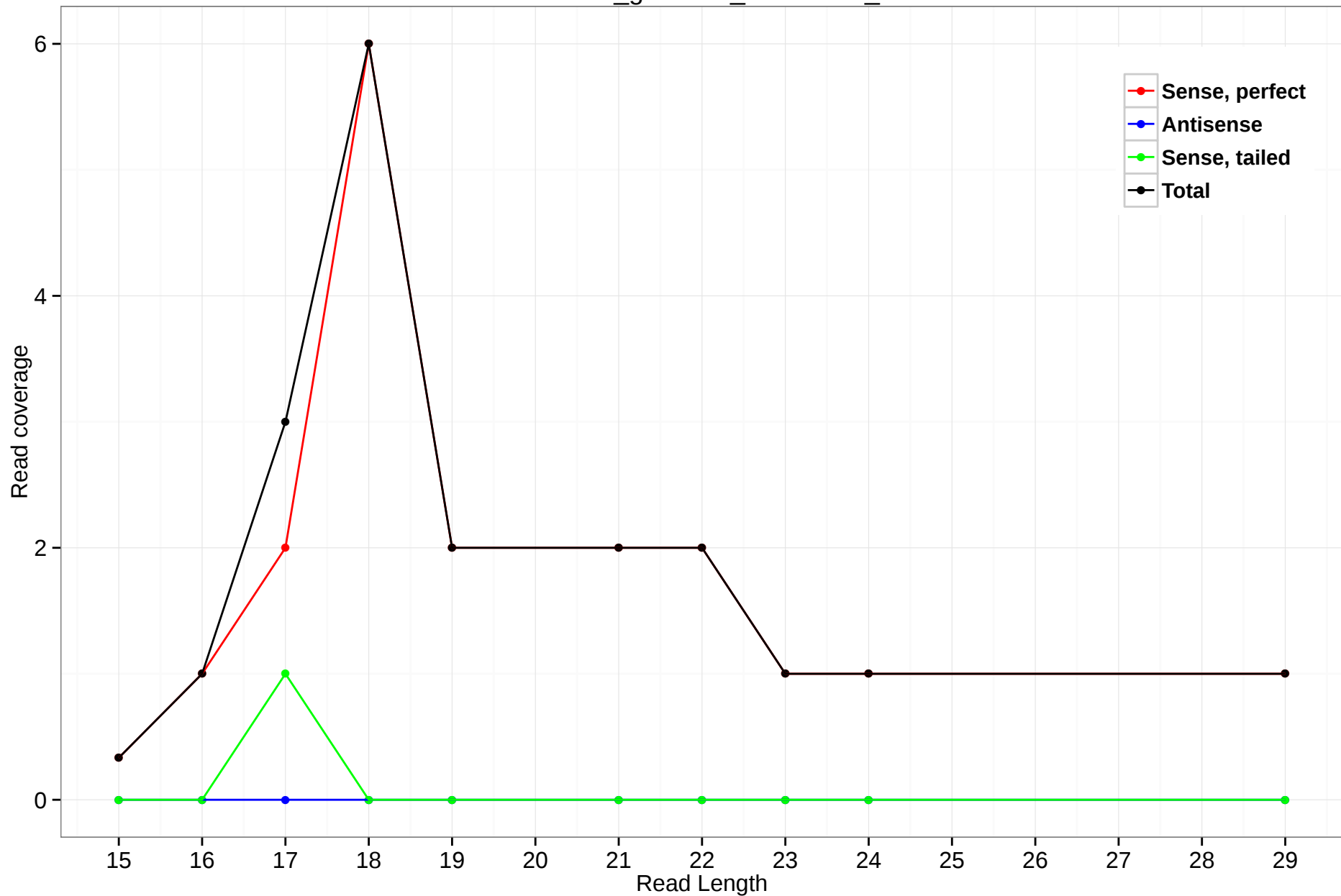
rheMac3_genscan_chr1.3434_8
