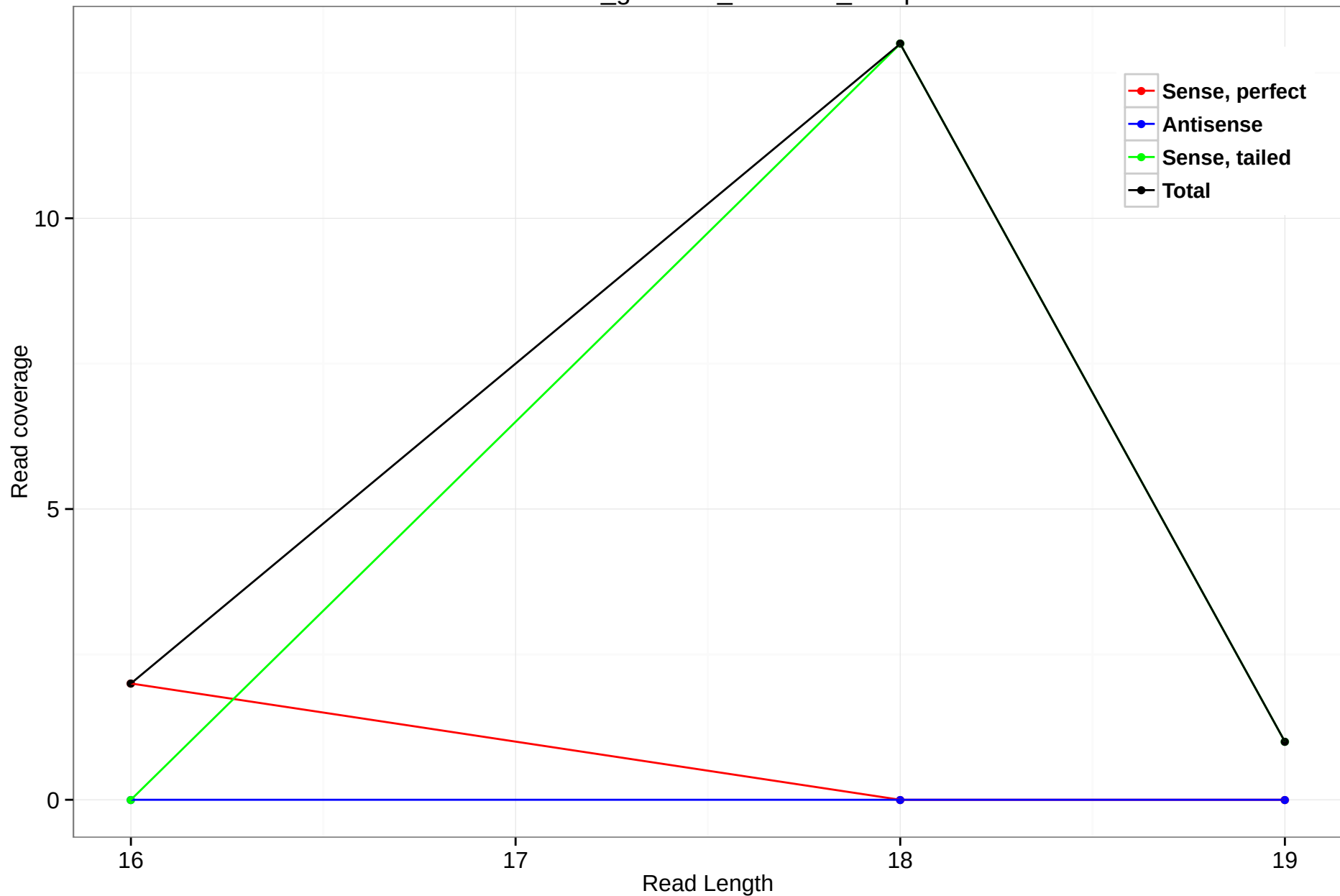
rheMac3_genscan_chr1.342_15.3p
