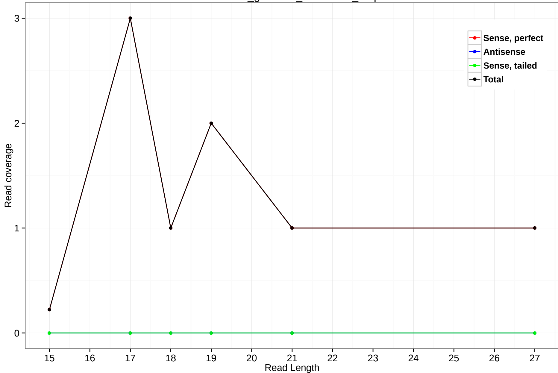
rheMac3_genscan_chr1.3396_1.3p
