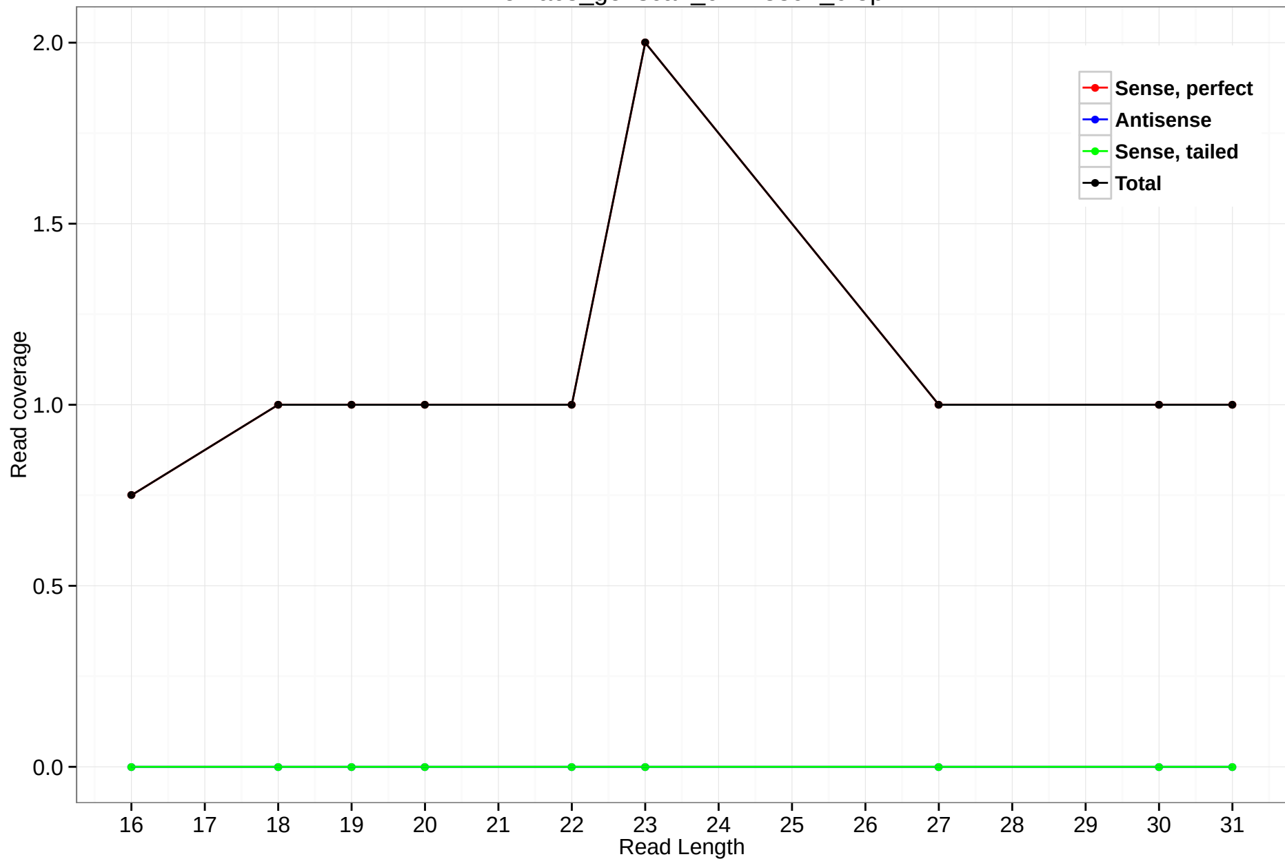
rheMac3_genscan_chr1.3394_0.5p
