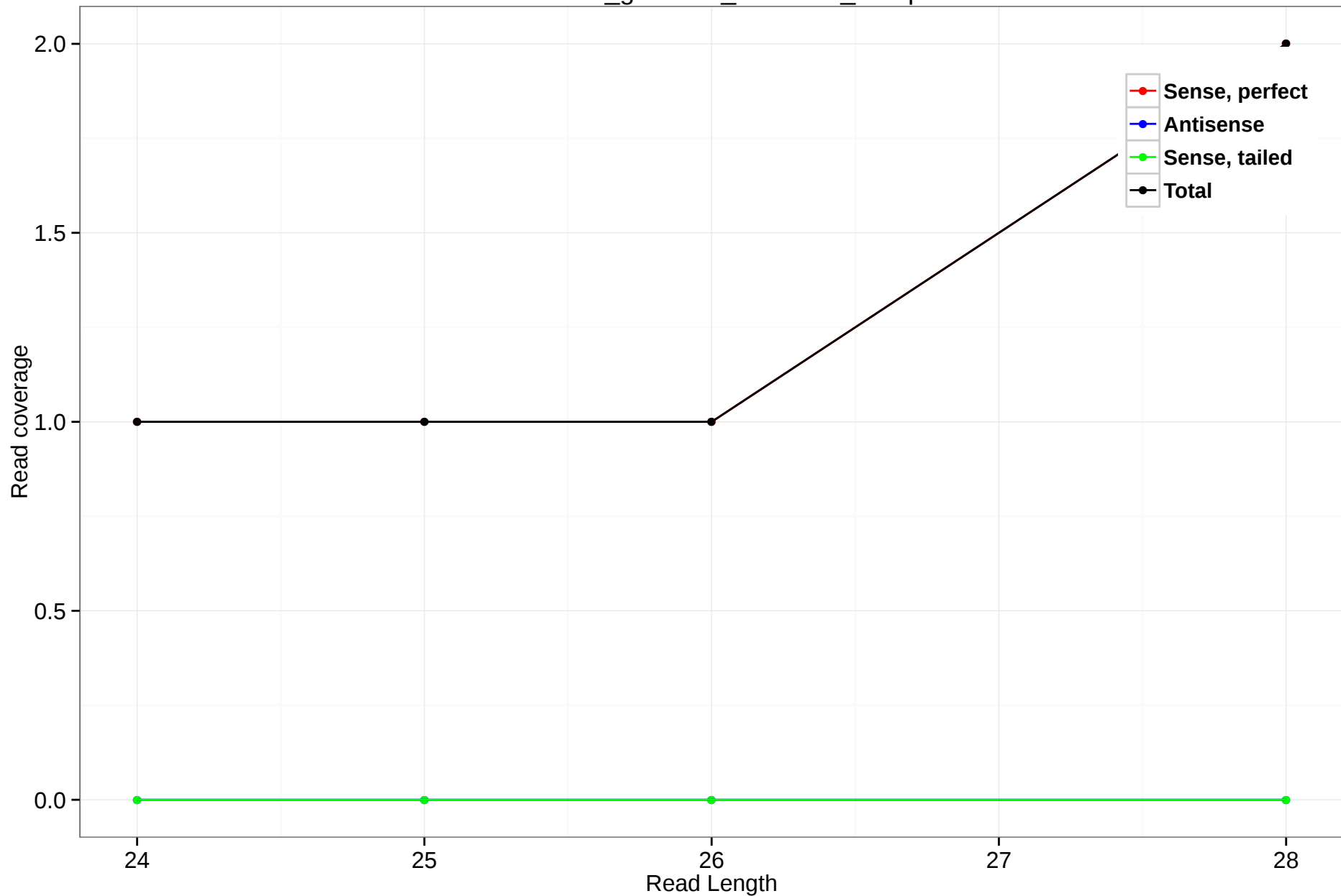
rheMac3_genscan_chr1.332_44.3p
