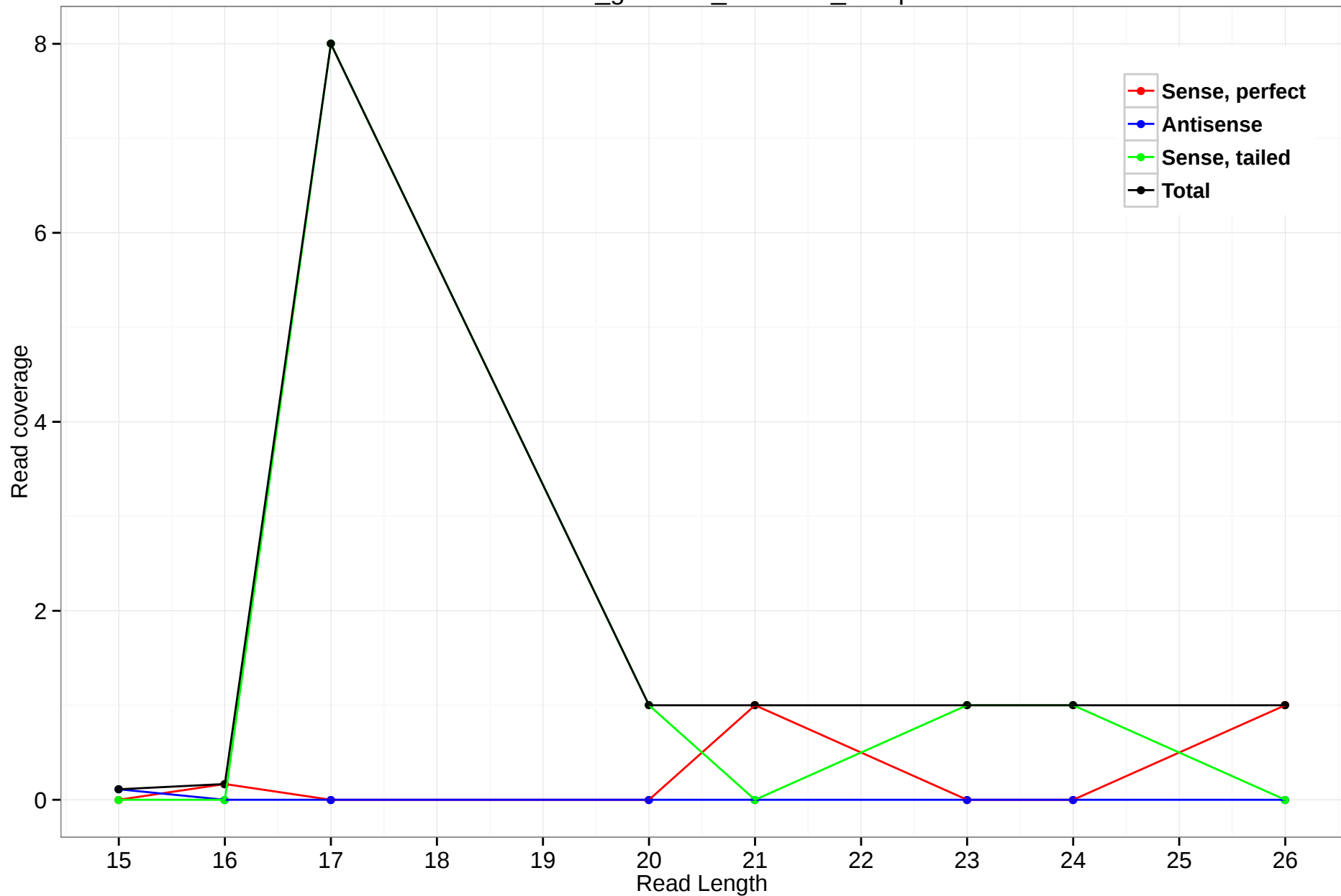
rheMac3_genscan_chr1.332_12.5p
