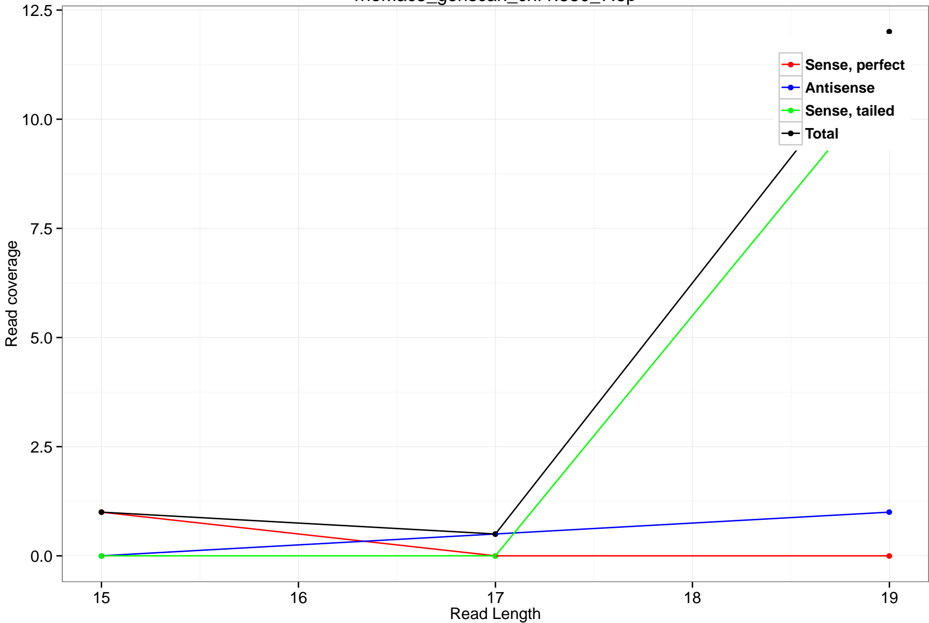
rheMac3_genscan_chr1.330_7.3p
