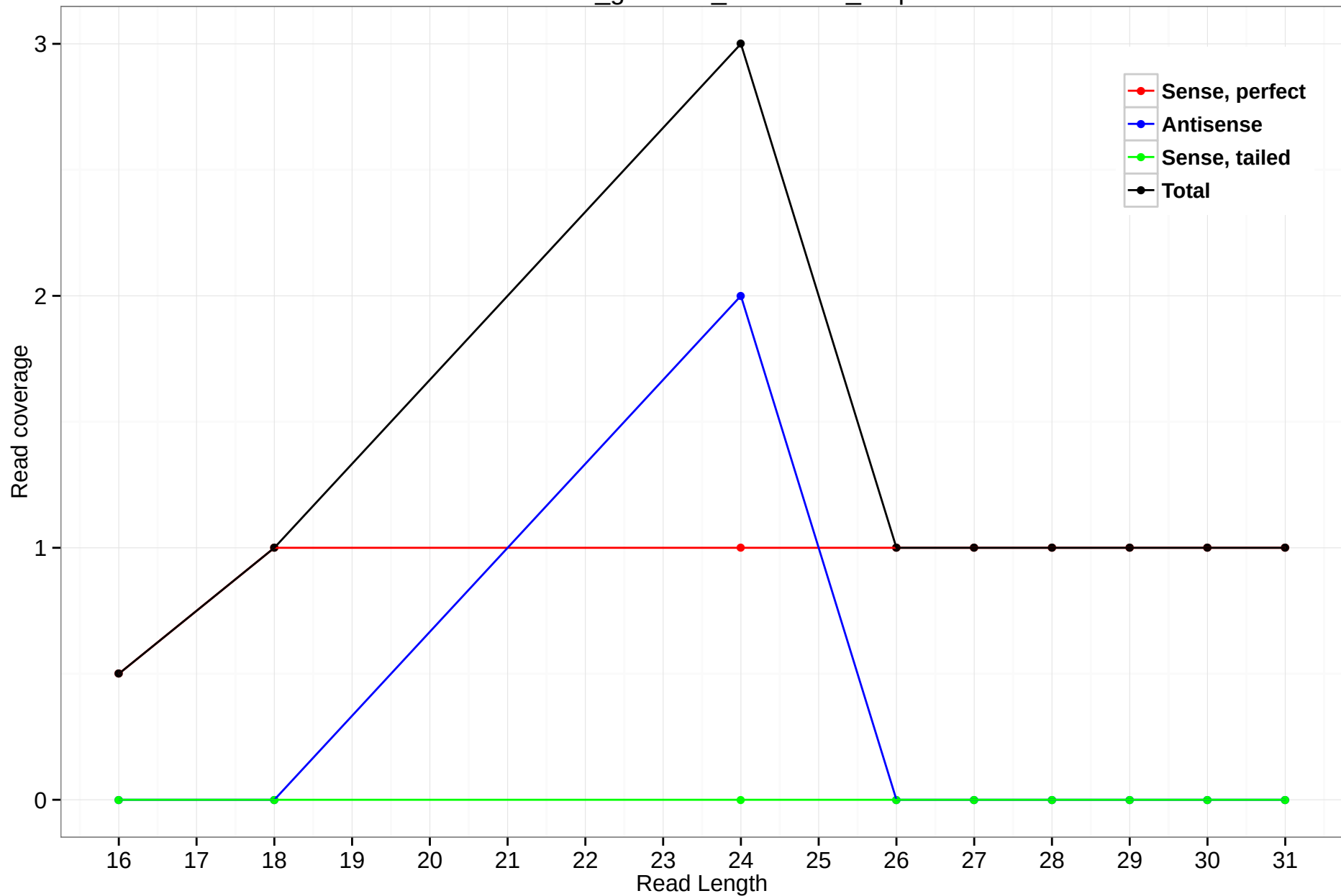
rheMac3_genscan_chr1.3258_1.5p
