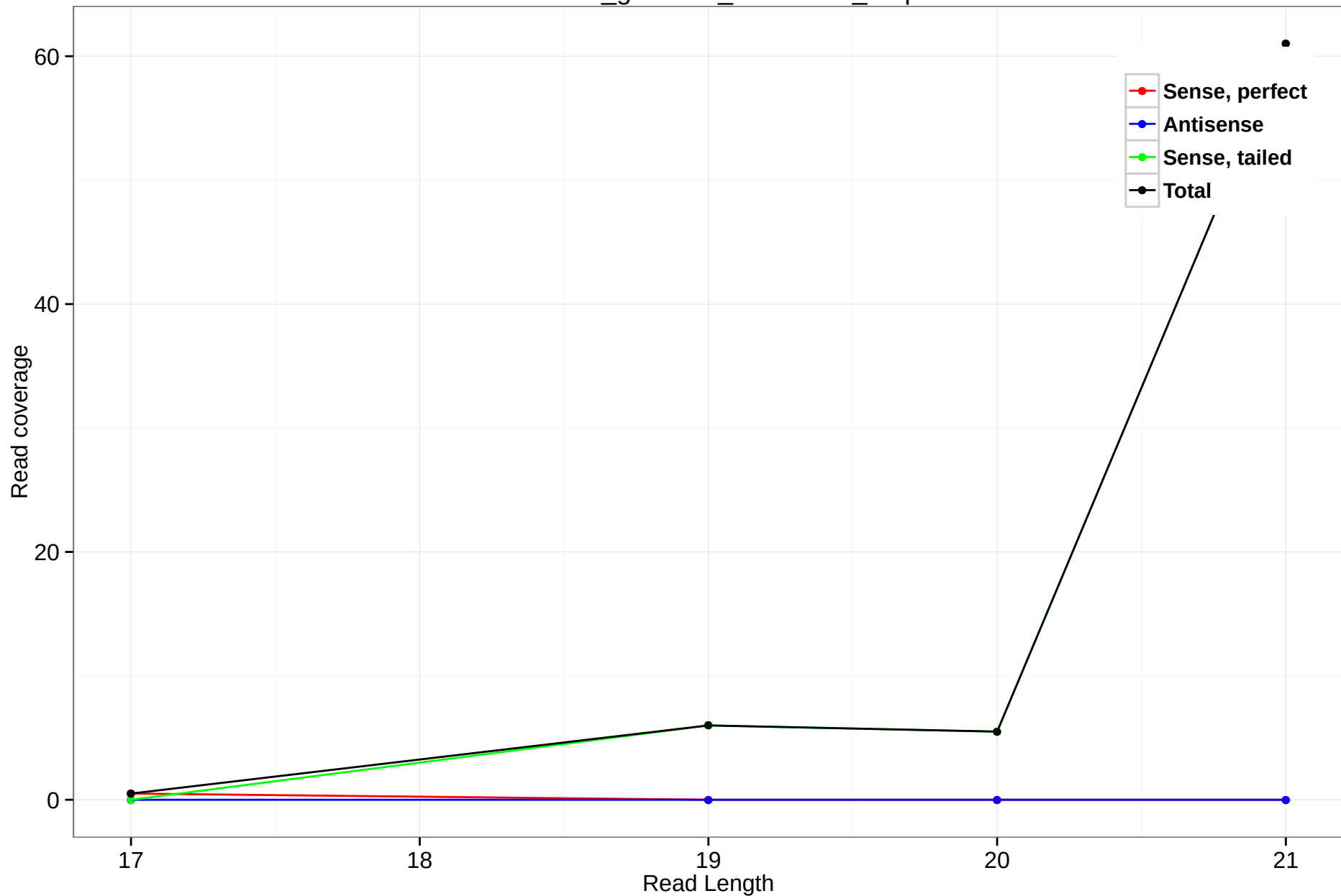
rheMac3_genscan_chr1.3235_8.3p
